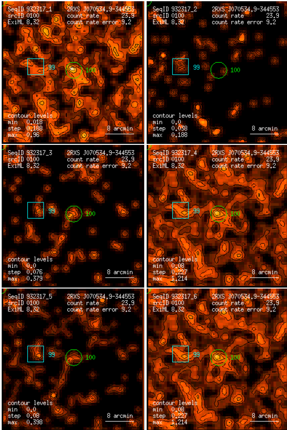
Figure 100: RASS 932317: detection 0100: band rate images, Gaussian filter: (1) PSPC channels 11 – 41, (2) 52 – 90, (3) 91 – 201, (4) 11 – 235, (5) 52 – 201, (6) 11 – 201. Broad band rates in counts/ks. Band rate contour levels in counts/ks/arcmin 2 .
