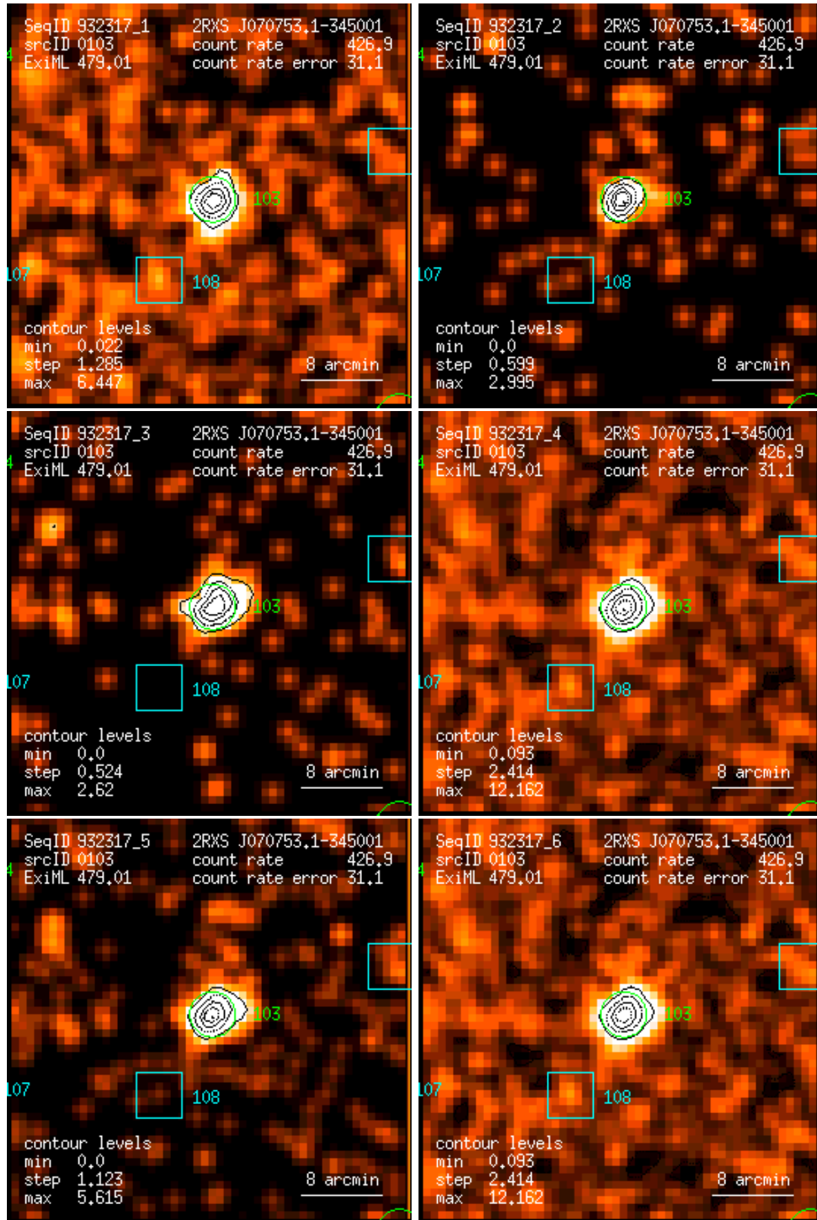
Figure 103: RASS 932317: detection 0103: band rate images, Gaussian filter: (1) PSPC channels 11 – 41, (2) 52 – 90, (3) 91 – 201, (4) 11 – 235, (5) 52 – 201, (6) 11 – 201. Broad band rates in counts/ks. Band rate contour levels in counts/ks/arcmin 2 .
