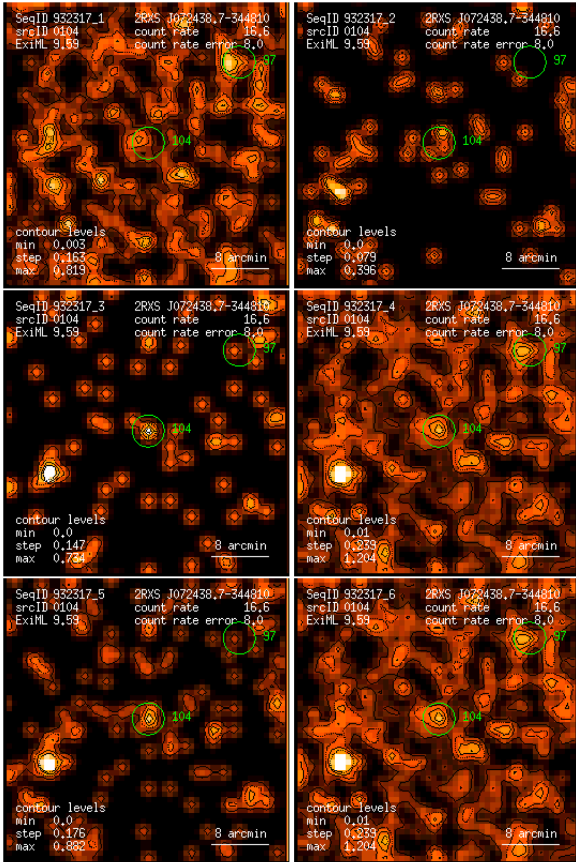
Figure 104: RASS 932317: detection 0104: band rate images, Gaussian filter: (1) PSPC channels 11 – 41, (2) 52 – 90, (3) 91 – 201, (4) 11 – 235, (5) 52 – 201, (6) 11 – 201. Broad band rates in counts/ks. Band rate contour levels in counts/ks/arcmin 2 .
