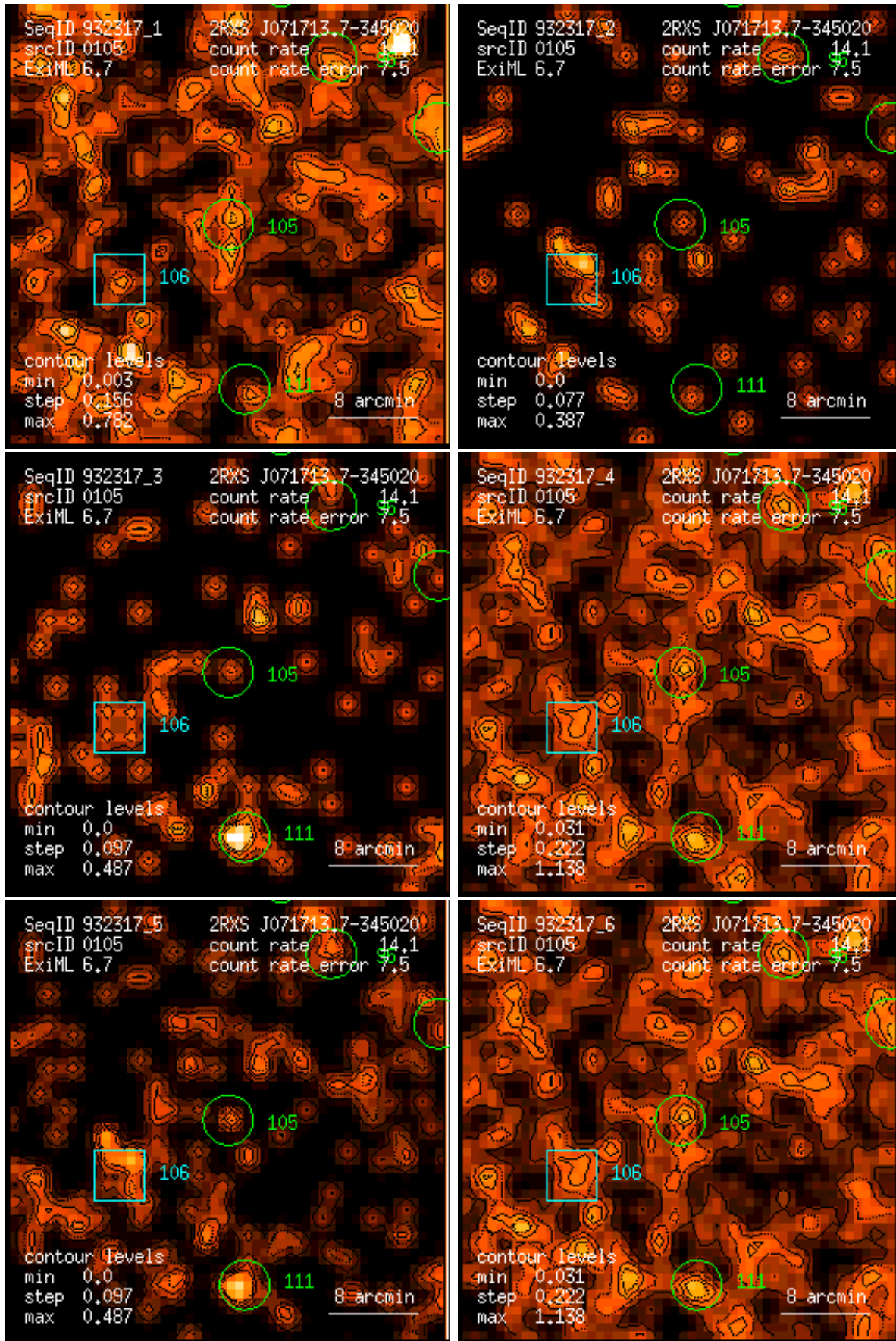
Figure 105: RASS 932317: detection 0105: band rate images, Gaussian filter: (1) PSPC channels 11 – 41, (2) 52 – 90, (3) 91 – 201, (4) 11 – 235, (5) 52 – 201, (6) 11 – 201. Broad band rates in counts/ks. Band rate contour levels in counts/ks/arcmin 2 .
