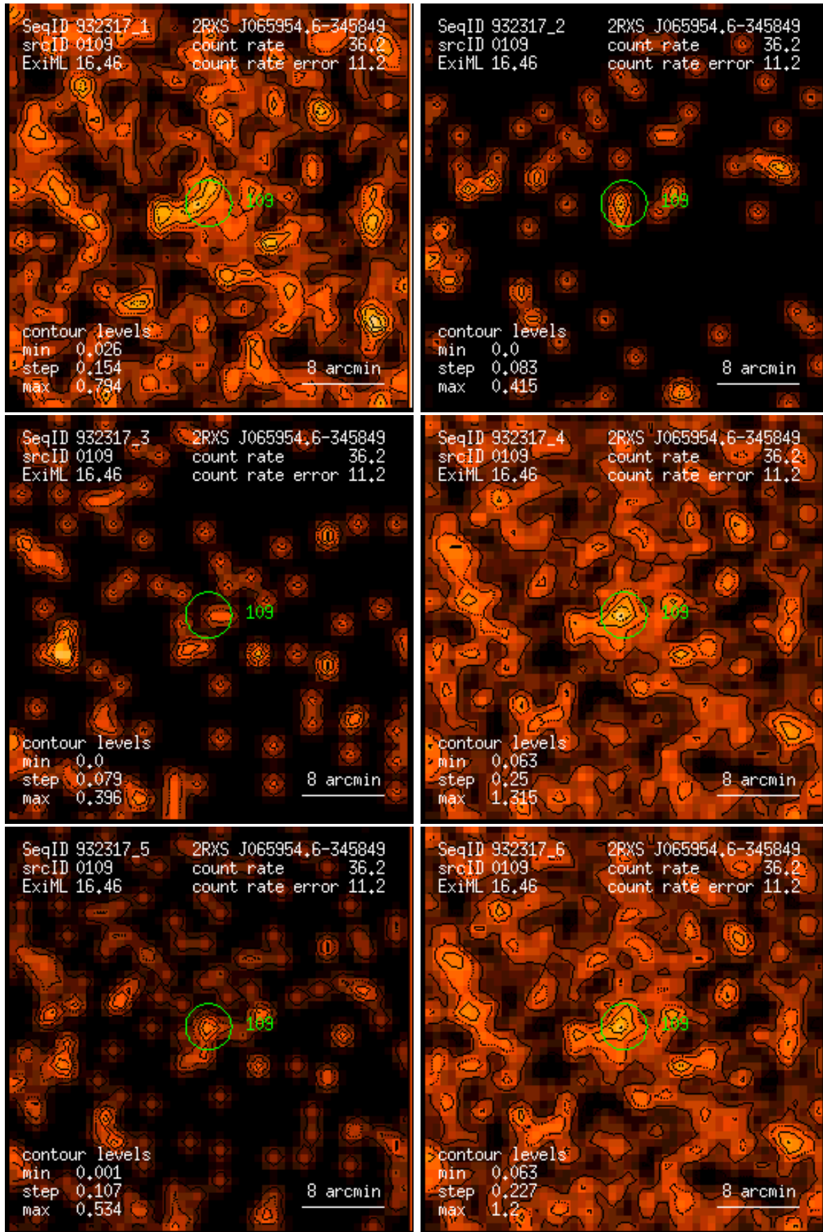
Figure 109: RASS 932317: detection 0109: band rate images, Gaussian filter: (1) PSPC channels 11 – 41, (2) 52 – 90, (3) 91 – 201, (4) 11 – 235, (5) 52 – 201, (6) 11 – 201. Broad band rates in counts/ks. Band rate contour levels in counts/ks/arcmin 2 .
