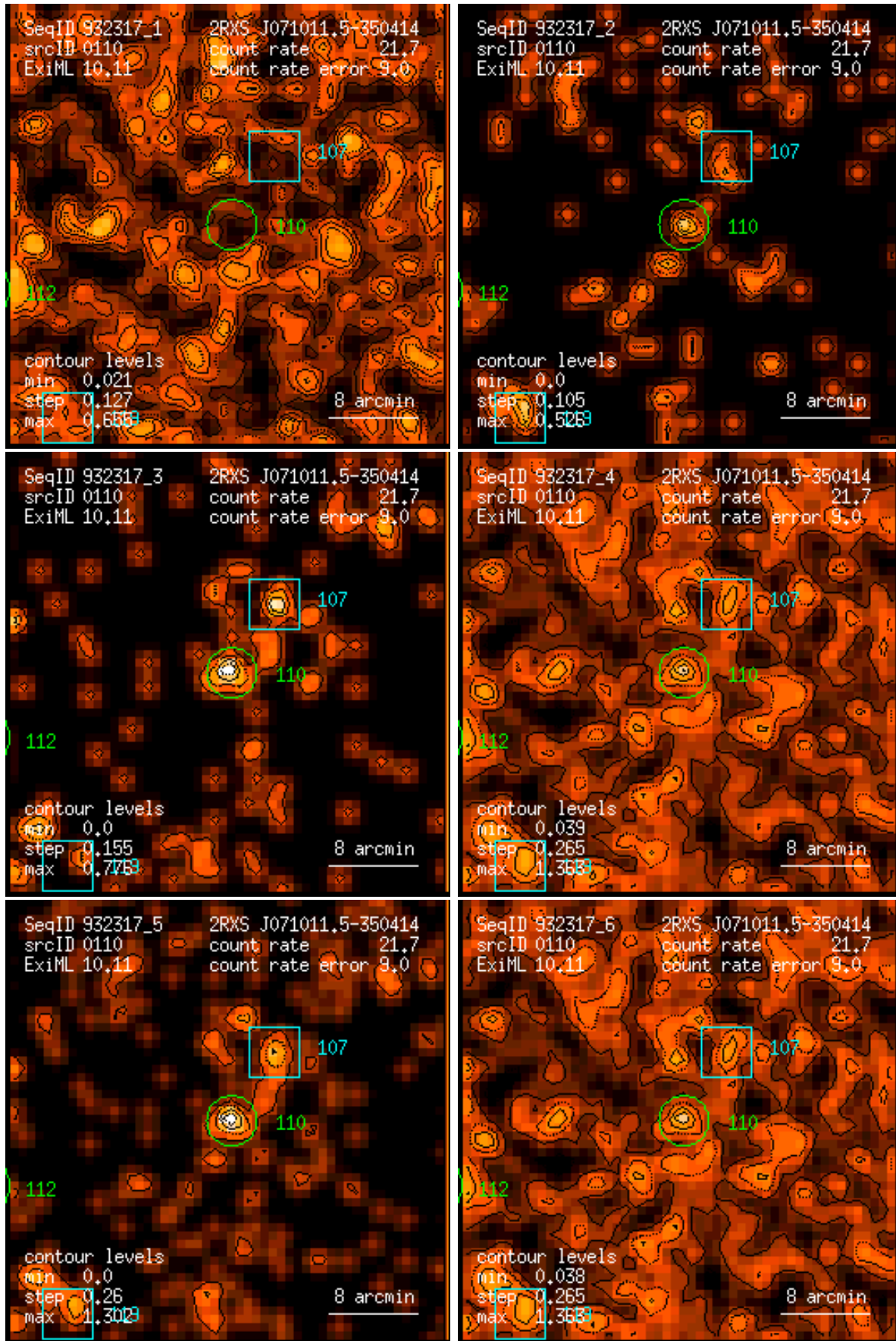
Figure 110: RASS 932317: detection 0110: band rate images, Gaussian filter: (1) PSPC channels 11 – 41, (2) 52 – 90, (3) 91 – 201, (4) 11 – 235, (5) 52 – 201, (6) 11 – 201. Broad band rates in counts/ks. Band rate contour levels in counts/ks/arcmin 2 .
