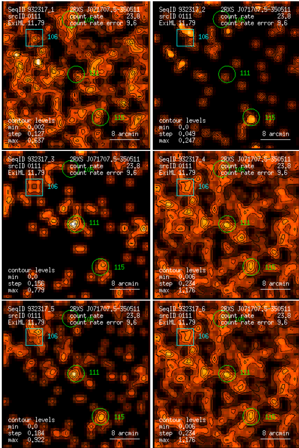
Figure 111: RASS 932317: detection 0111: band rate images, Gaussian filter: (1) PSPC channels 11 – 41, (2) 52 – 90, (3) 91 – 201, (4) 11 – 235, (5) 52 – 201, (6) 11 – 201. Broad band rates in counts/ks. Band rate contour levels in counts/ks/arcmin 2 .
