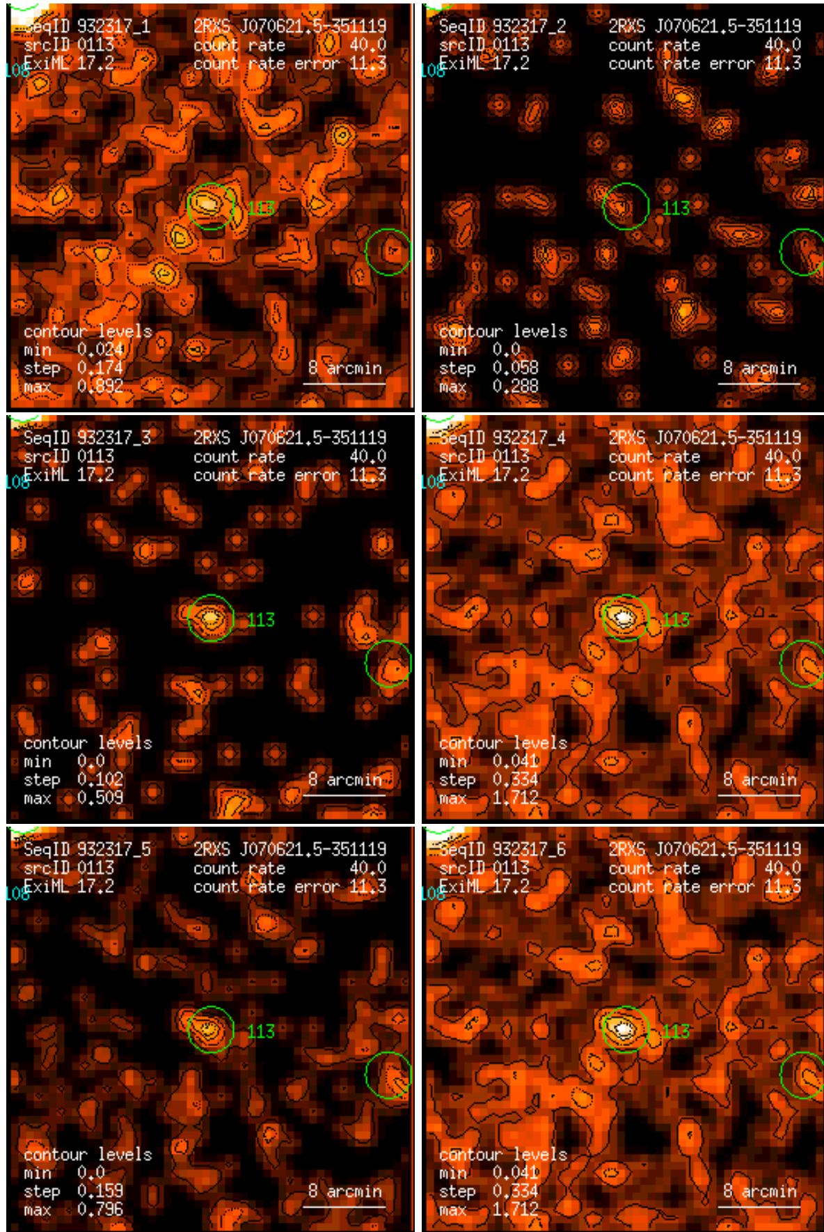
Figure 113: RASS 932317: detection 0113: band rate images, Gaussian filter: (1) PSPC channels 11 – 41, (2) 52 – 90, (3) 91 – 201, (4) 11 – 235, (5) 52 – 201, (6) 11 – 201. Broad band rates in counts/ks. Band rate contour levels in counts/ks/arcmin 2 .
