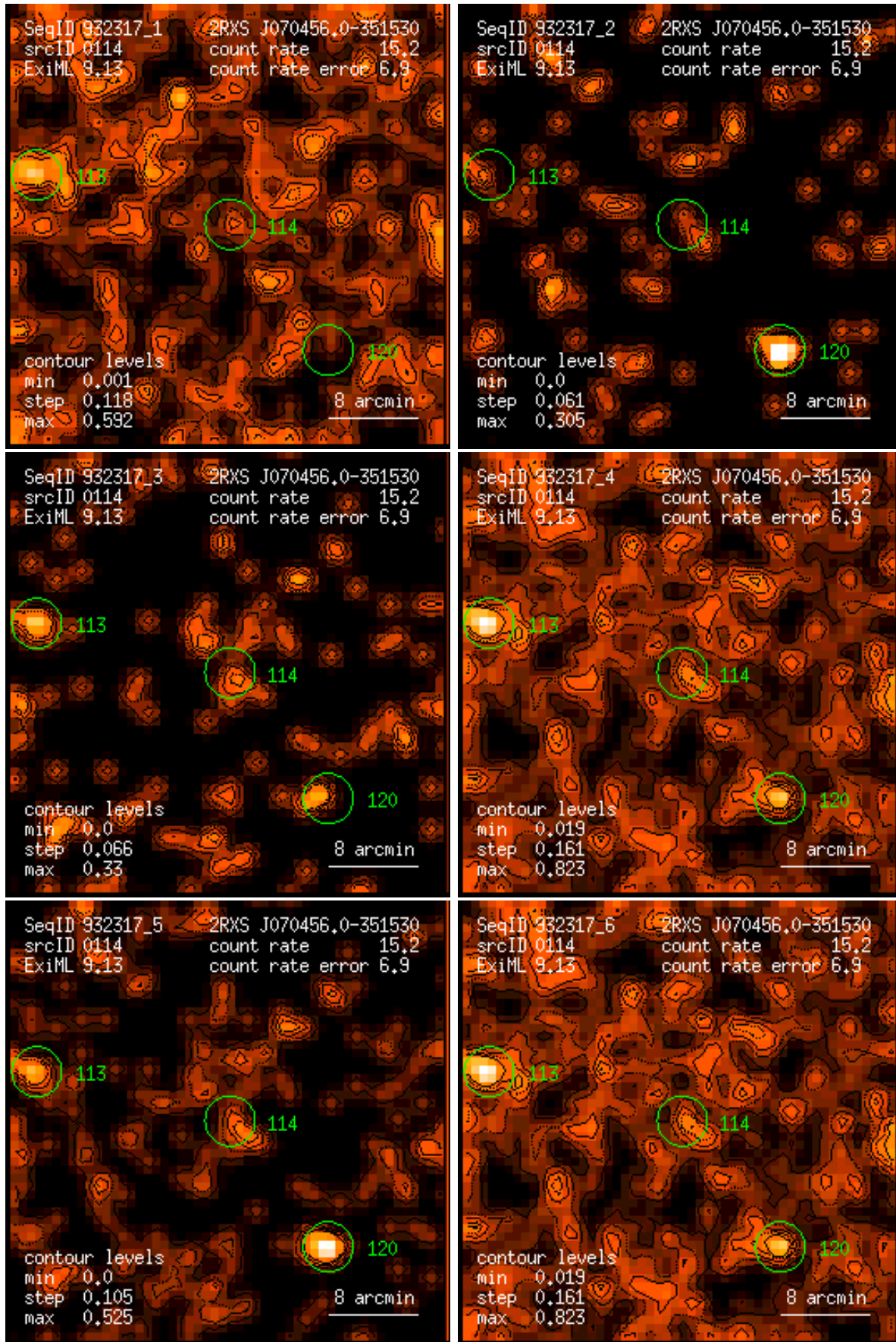
Figure 114: RASS 932317: detection 0114: band rate images, Gaussian filter: (1) PSPC channels 11 – 41, (2) 52 – 90, (3) 91 – 201, (4) 11 – 235, (5) 52 – 201, (6) 11 – 201. Broad band rates in counts/ks. Band rate contour levels in counts/ks/arcmin 2 .
