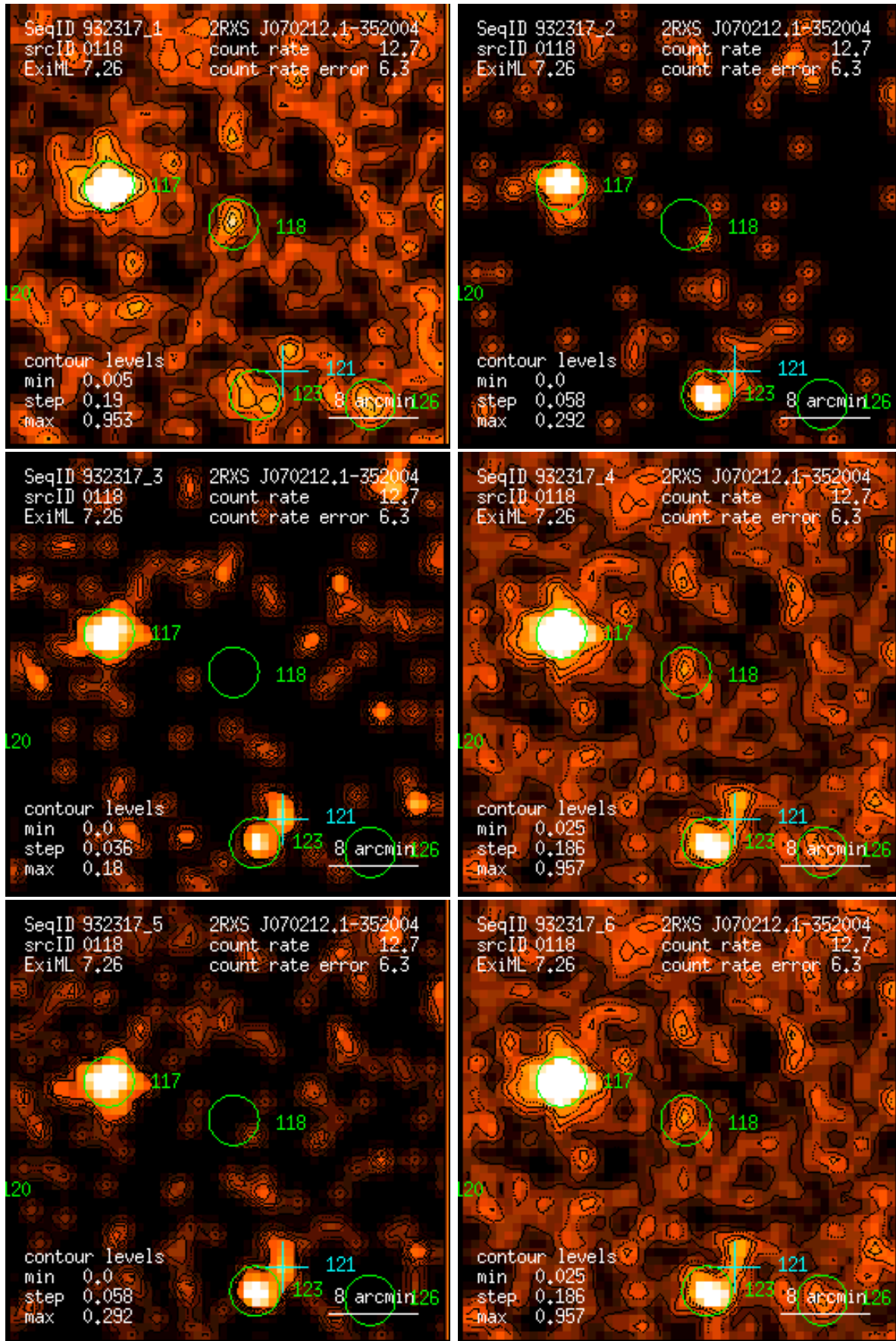
Figure 118: RASS 932317: detection 0118: band rate images, Gaussian filter: (1) PSPC channels 11 – 41, (2) 52 – 90, (3) 91 – 201, (4) 11 – 235, (5) 52 – 201, (6) 11 – 201. Broad band rates in counts/ks. Band rate contour levels in counts/ks/arcmin 2 .
