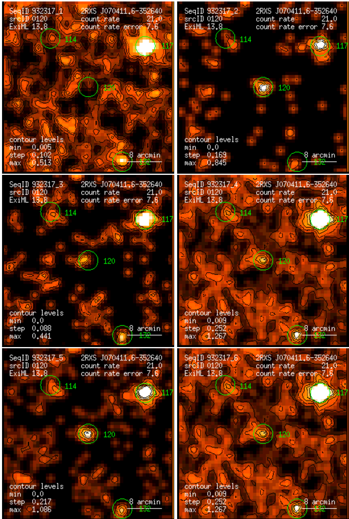
Figure 120: RASS 932317: detection 0120: band rate images, Gaussian filter: (1) PSPC channels 11 – 41, (2) 52 – 90, (3) 91 – 201, (4) 11 – 235, (5) 52 – 201, (6) 11 – 201. Broad band rates in counts/ks. Band rate contour levels in counts/ks/arcmin 2 .
