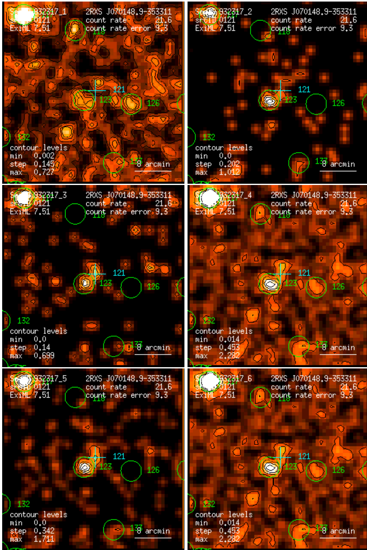
Figure 121: RASS 932317: detection 0121: band rate images, Gaussian filter: (1) PSPC channels 11 – 41, (2) 52 – 90, (3) 91 – 201, (4) 11 – 235, (5) 52 – 201, (6) 11 – 201. Broad band rates in counts/ks. Band rate contour levels in counts/ks/arcmin 2 .
