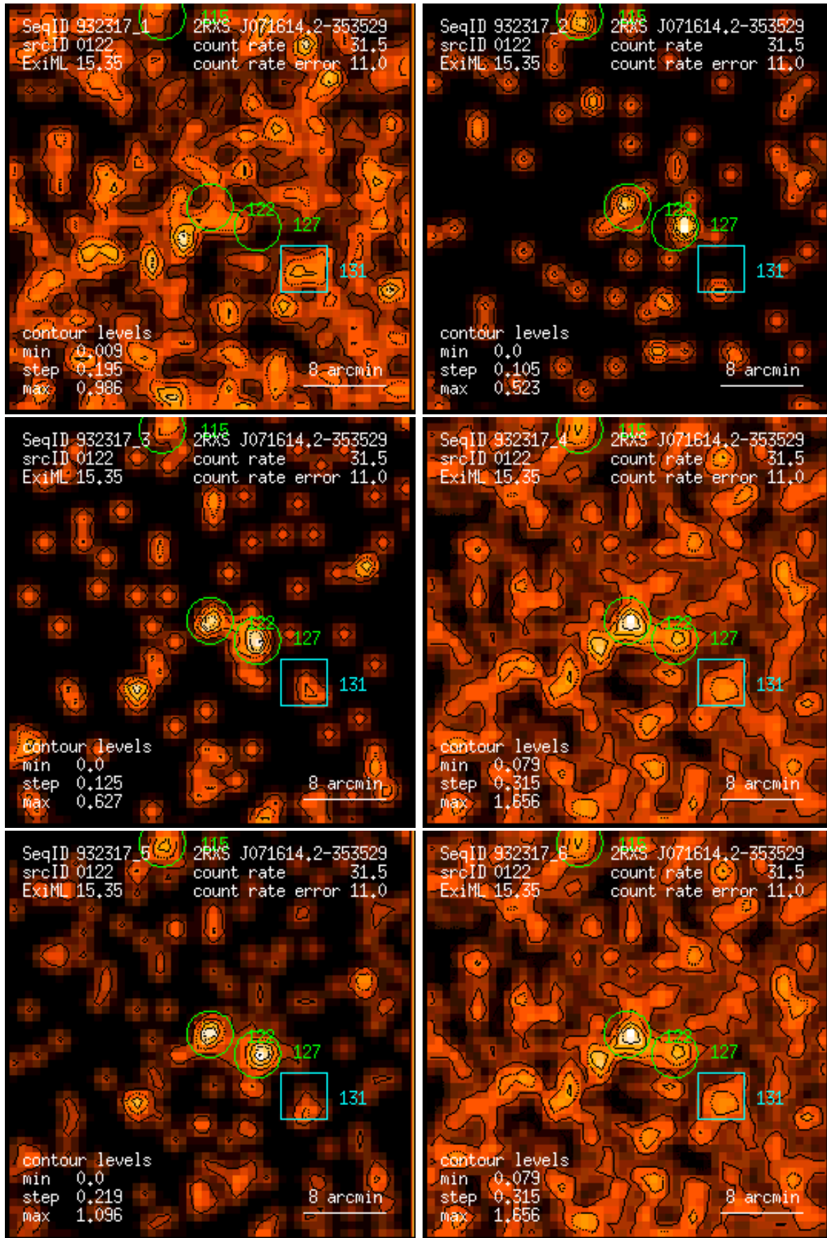
Figure 122: RASS 932317: detection 0122: band rate images, Gaussian filter: (1) PSPC channels 11 – 41, (2) 52 – 90, (3) 91 – 201, (4) 11 – 235, (5) 52 – 201, (6) 11 – 201. Broad band rates in counts/ks. Band rate contour levels in counts/ks/arcmin 2 .
