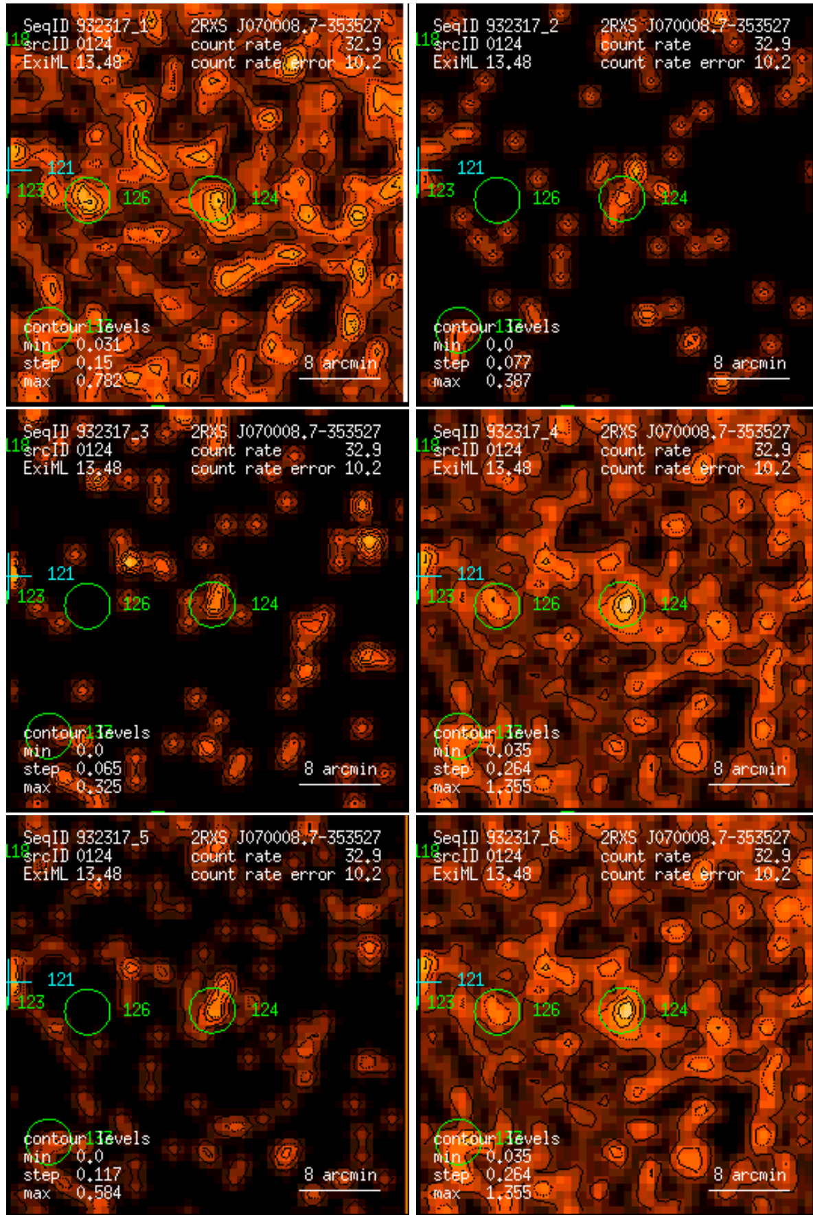
Figure 124: RASS 932317: detection 0124: band rate images, Gaussian filter: (1) PSPC channels 11 – 41, (2) 52 – 90, (3) 91 – 201, (4) 11 – 235, (5) 52 – 201, (6) 11 – 201. Broad band rates in counts/ks. Band rate contour levels in counts/ks/arcmin 2 .
