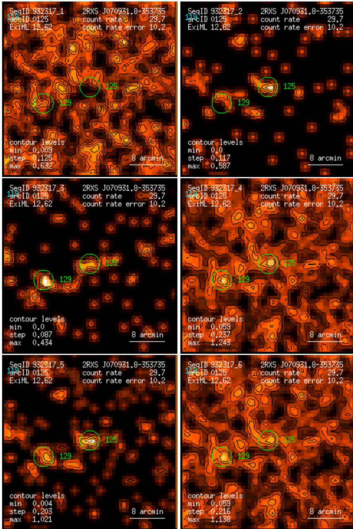
Figure 125: RASS 932317: detection 0125: band rate images, Gaussian filter: (1) PSPC channels 11 – 41, (2) 52 – 90, (3) 91 – 201, (4) 11 – 235, (5) 52 – 201, (6) 11 – 201. Broad band rates in counts/ks. Band rate contour levels in counts/ks/arcmin 2 .
