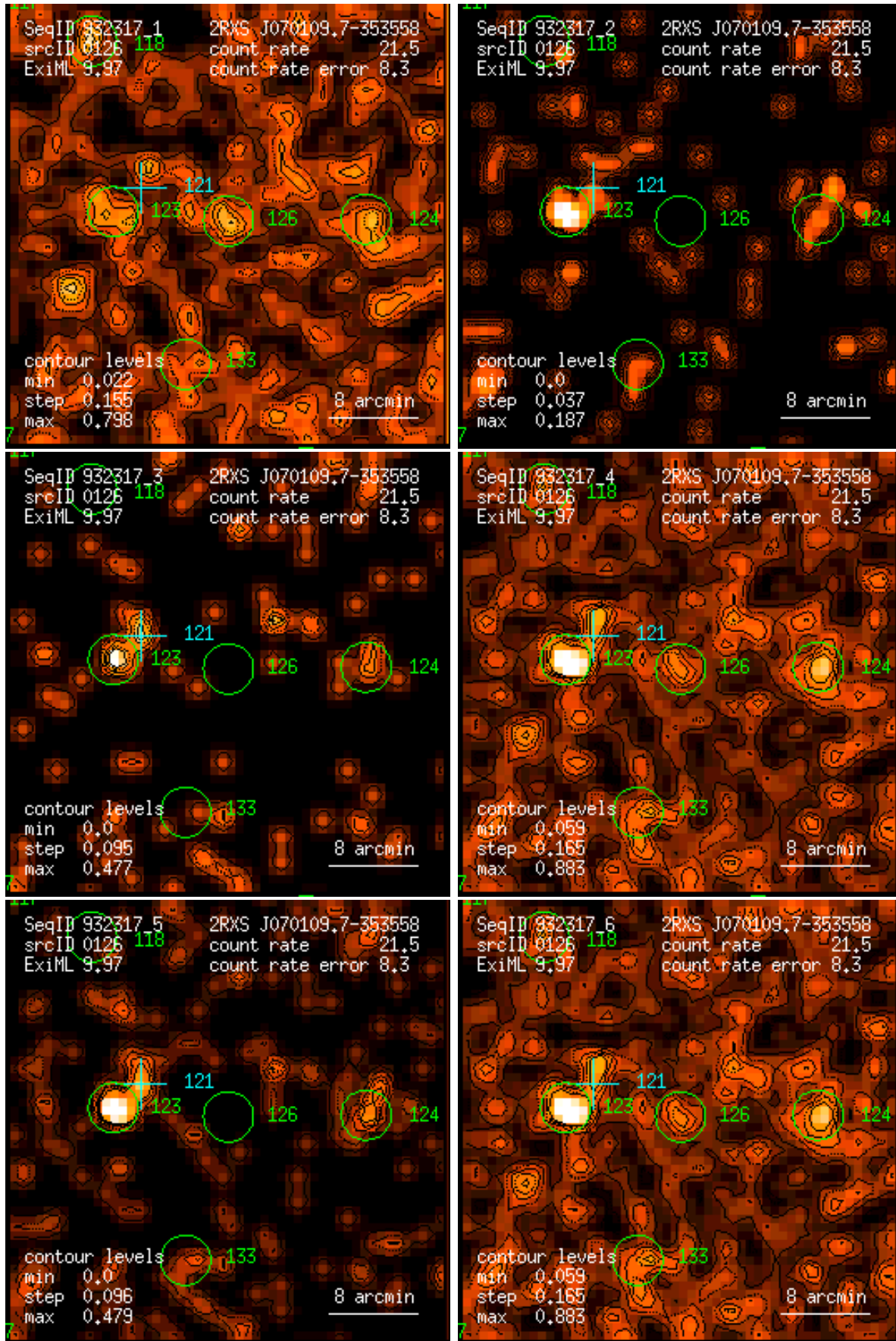
Figure 126: RASS 932317: detection 0126: band rate images, Gaussian filter: (1) PSPPC channels 11 – 41, (2) 52 – 90, (3) 91 – 201, (4) 11 – 235, (5) 52 – 201, (6) 11 – 201. Broad band rates in counts/ks. Band rate contour levels in counts/ks/arcmin 2 .
