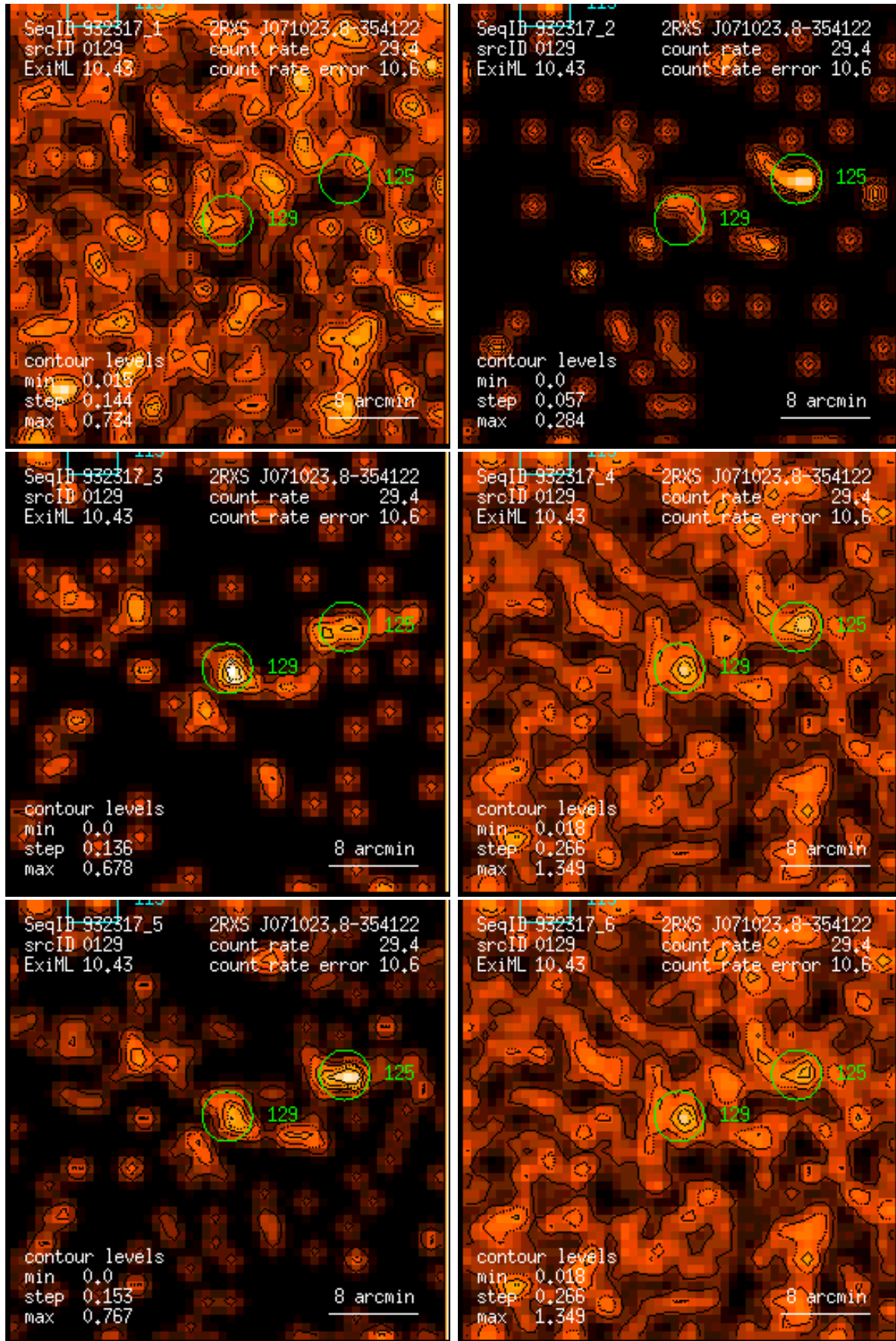
Figure 129: RASS 932317: detection 0129: band rate images, Gaussian filter: (1) PSPC channels 11 – 41, (2) 52 – 90, (3) 91 – 201, (4) 11 – 235, (5) 52 – 201, (6) 11 – 201. Broad band rates in counts/ks. Band rate contour levels in counts/ks/arcmin 2 .
