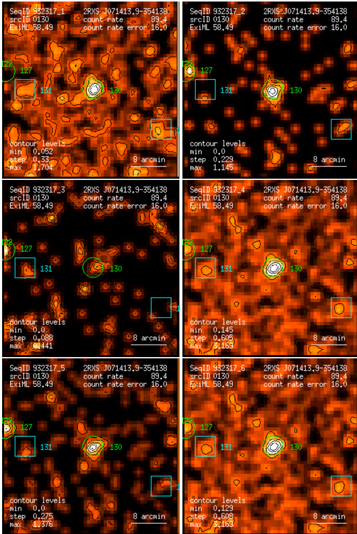
Figure 130: RASS 932317: detection 0130: band rate images, Gaussian filter: (1) PSPC channels 11 – 41, (2) 52 – 90, (3) 91 – 201, (4) 11 – 235, (5) 52 – 201, (6) 11 – 201. Broad band rates in counts/ks. Band rate contour levels in counts/ks/arcmin 2 .
