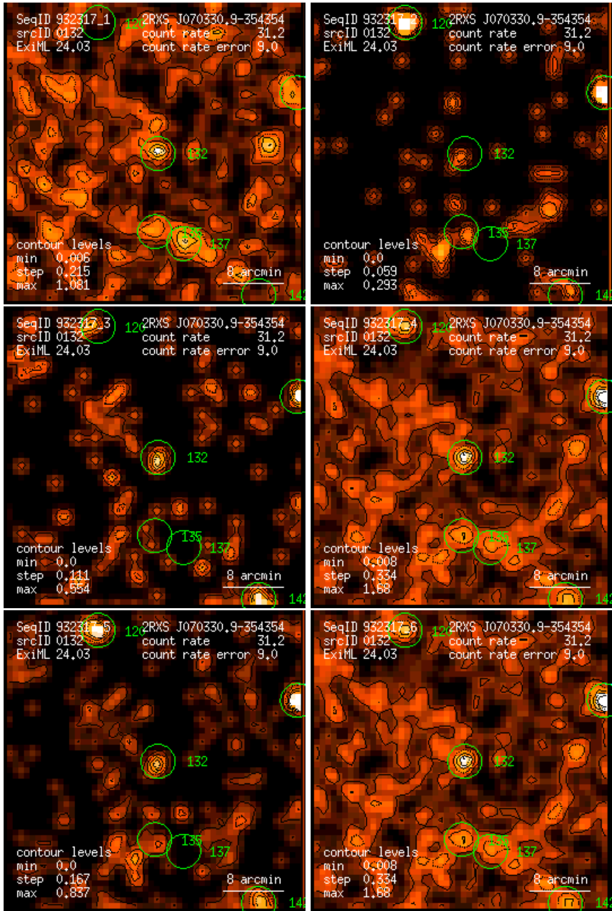
Figure 132: RASS 932317: detection 0132: band rate images, Gaussian filter: (1) PSPC channels 11 – 41, (2) 52 – 90, (3) 91 – 201, (4) 11 – 235, (5) 52 – 201, (6) 11 – 201. Broad band rates in counts/ks. Band rate contour levels in counts/ks/arcmin 2 .
