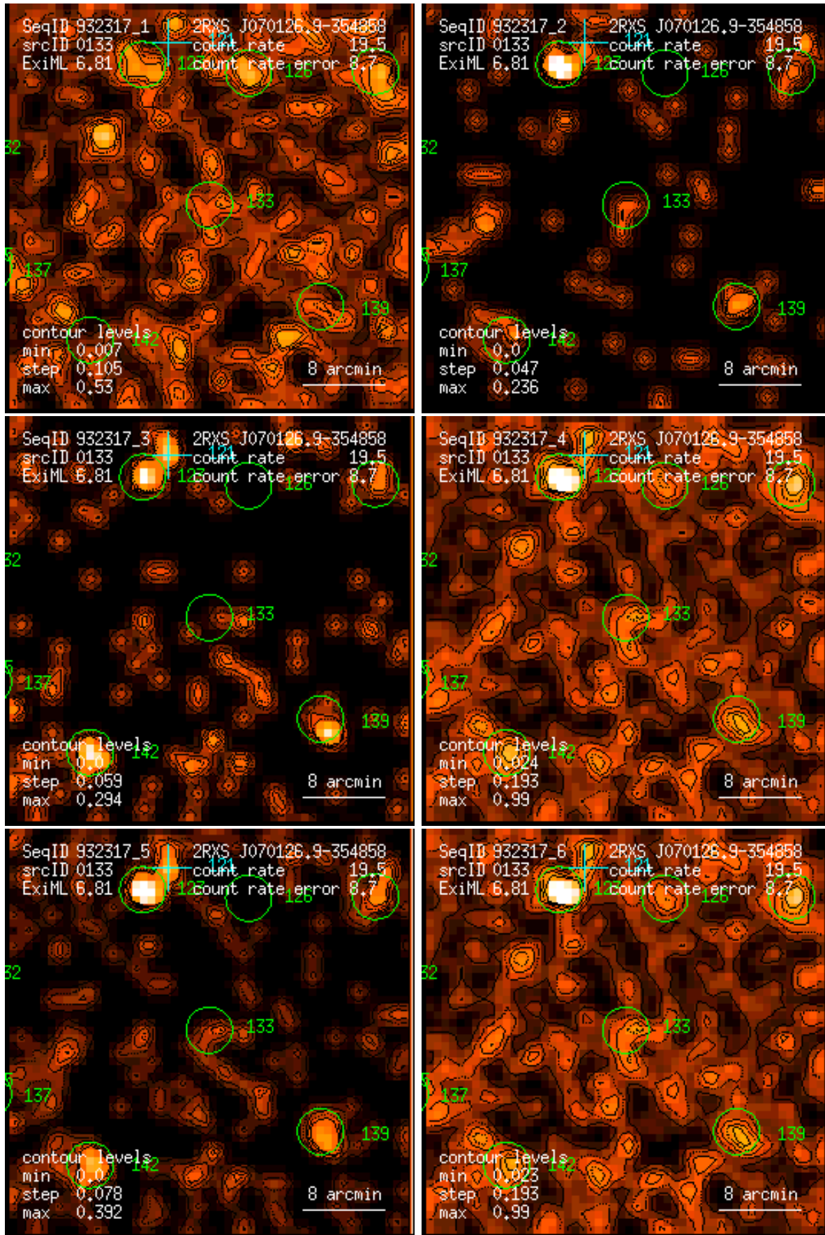
Figure 133: RASS 932317: detection 0133: band rate images, Gaussian filter: (1) PSPC channels 11 – 41, (2) 52 – 90, (3) 91 – 201, (4) 11 – 235, (5) 52 – 201, (6) 11 – 201. Broad band rates in counts/ks. Band rate contour levels in counts/ks/arcmin 2 .
