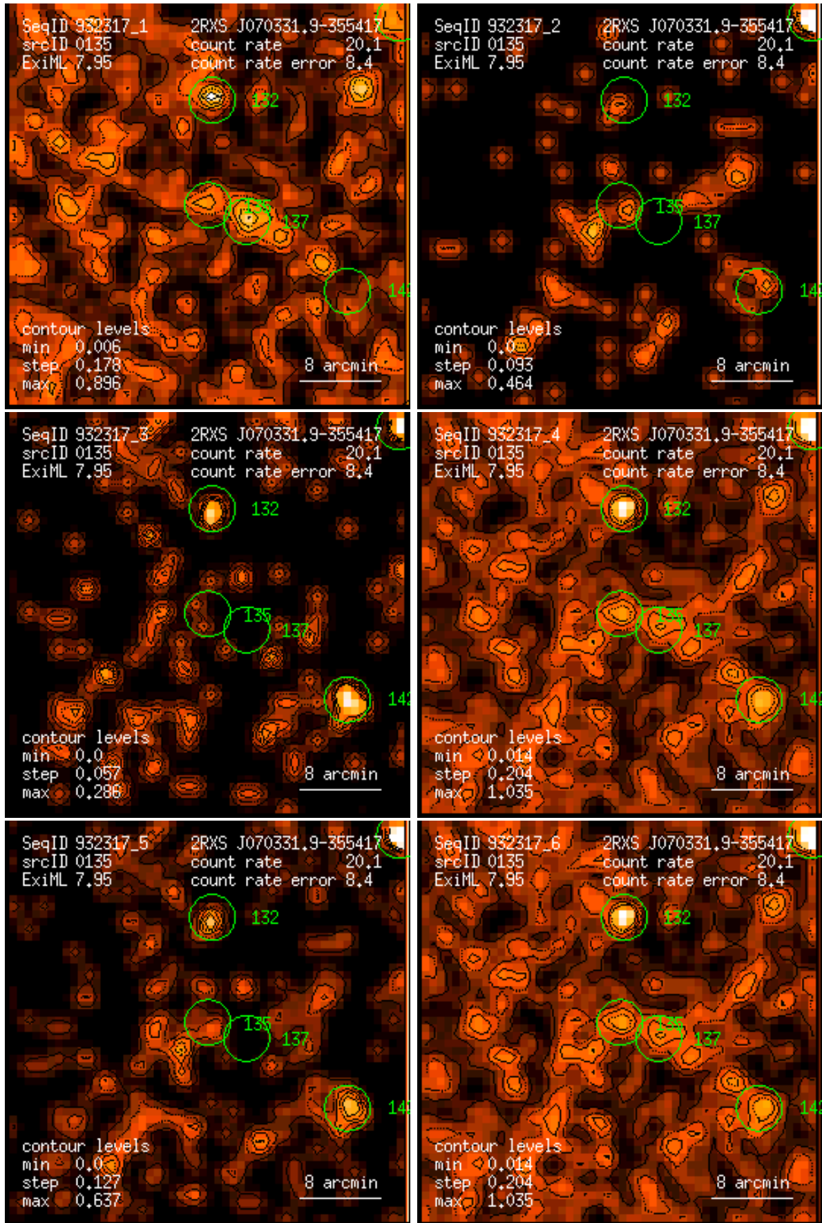
Figure 135: RASS 932317: detection 0135: band rate images, Gaussian filter: (1) PSPC channels 11 – 41, (2) 52 – 90, (3) 91 – 201, (4) 11 – 235, (5) 52 – 201, (6) 11 – 201. Broad band rates in counts/ks. Band rate contour levels in counts/ks/arcmin 2 .
