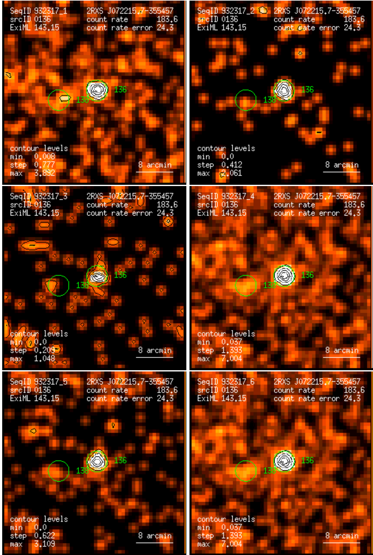
Figure 136: RASS 932317: detection 0136: band rate images, Gaussian filter: (1) PSPC channels 11 – 41, (2) 52 – 90, (3) 91 – 201, (4) 11 – 235, (5) 52 – 201, (6) 11 – 201. Broad band rates in counts/ks. Band rate contour levels in counts/ks/arcmin 2 .
