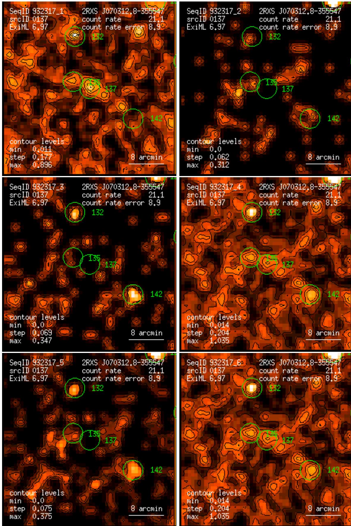
Figure 137: RASS 932317: detection 0137: band rate images, Gaussian filter: (1) PSPC channels 11 – 41, (2) 52 – 90, (3) 91 – 201, (4) 11 – 235, (5) 52 – 201, (6) 11 – 201. Broad band rates in counts/ks. Band rate contour levels in counts/ks/arcmin 2 .
