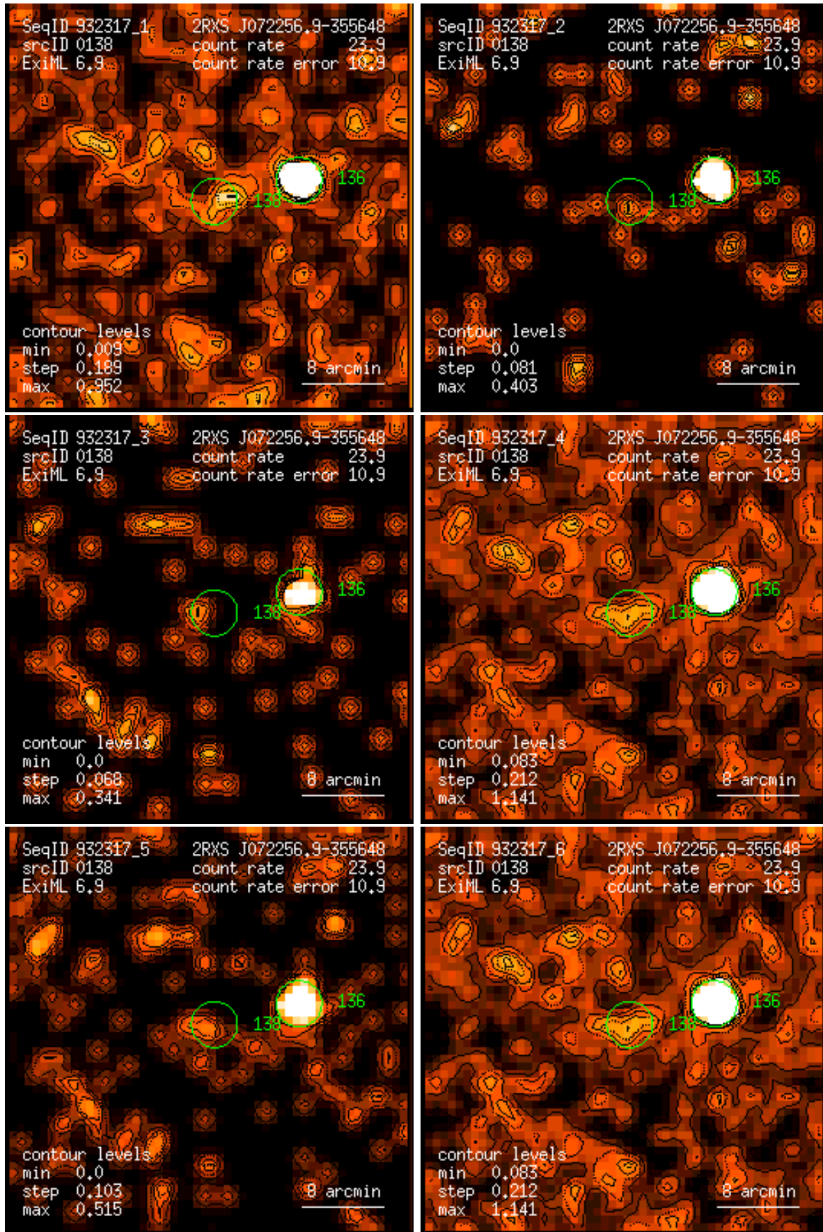
Figure 138: RASS 932317: detection 0138: band rate images, Gaussian filter: (1) PSPC channels 11 – 41, (2) 52 – 90, (3) 91 – 201, (4) 11 – 235, (5) 52 – 201, (6) 11 – 201. Broad band rates in counts/ks. Band rate contour levels in counts/ks/arcmin 2 .
