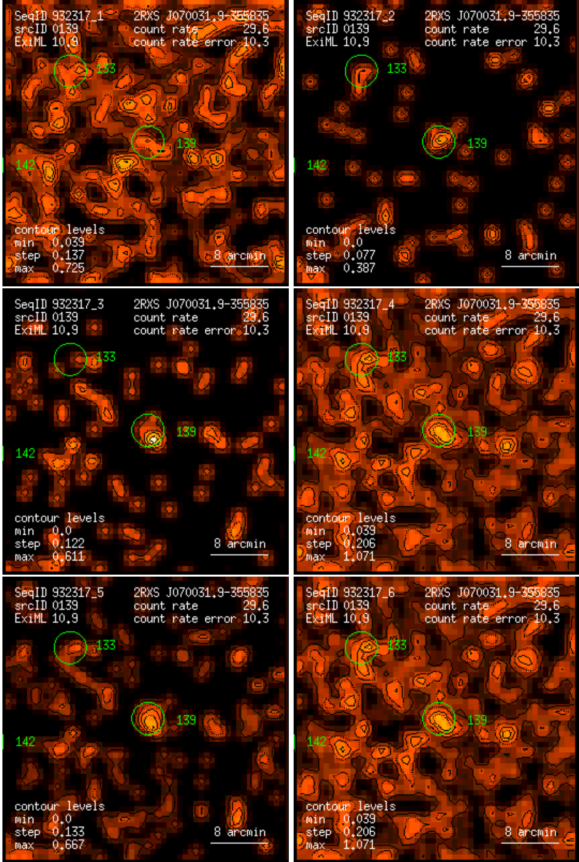
Figure 139: RASS 932317: detection 0139: band rate images, Gaussian filter: (1) PSPC channels 11 – 41, (2) 52 – 90, (3) 91 – 201, (4) 11 – 235, (5) 52 – 201, (6) 11 – 201. Broad band rates in counts/ks. Band rate contour levels in counts/ks/arcmin 2 .
