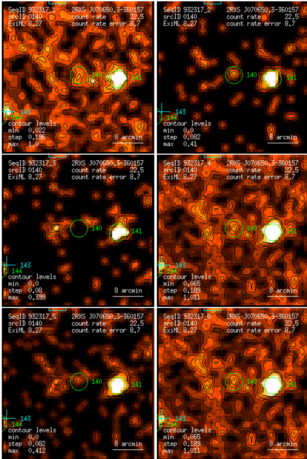
Figure 140: RASS 932317: detection 0140: band rate images, Gaussian filter: (1) PSPC channels 11 – 41, (2) 52 – 90, (3) 91 – 201, (4) 11 – 235, (5) 52 – 201, (6) 11 – 201. Broad band rates in counts/ks. Band rate contour levels in counts/ks/arcmin 2 .
