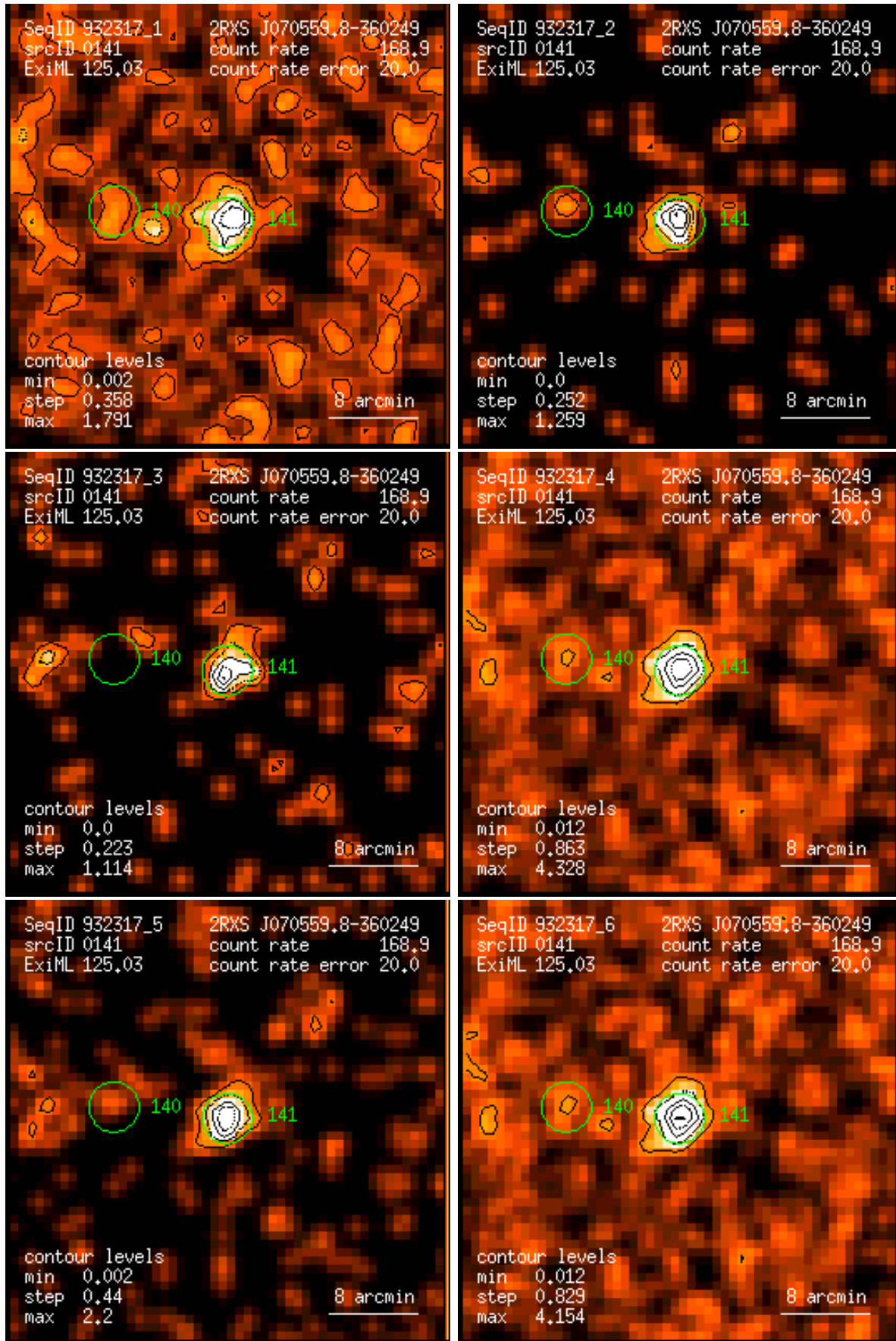
Figure 141: RASS 932317: detection 0141: band rate images, Gaussian filter: (1) PSPC channels 11 – 41, (2) 52 – 90, (3) 91 – 201, (4) 11 – 235, (5) 52 – 201, (6) 11 – 201. Broad band rates in counts/ks. Band rate contour levels in counts/ks/arcmin 2 .
