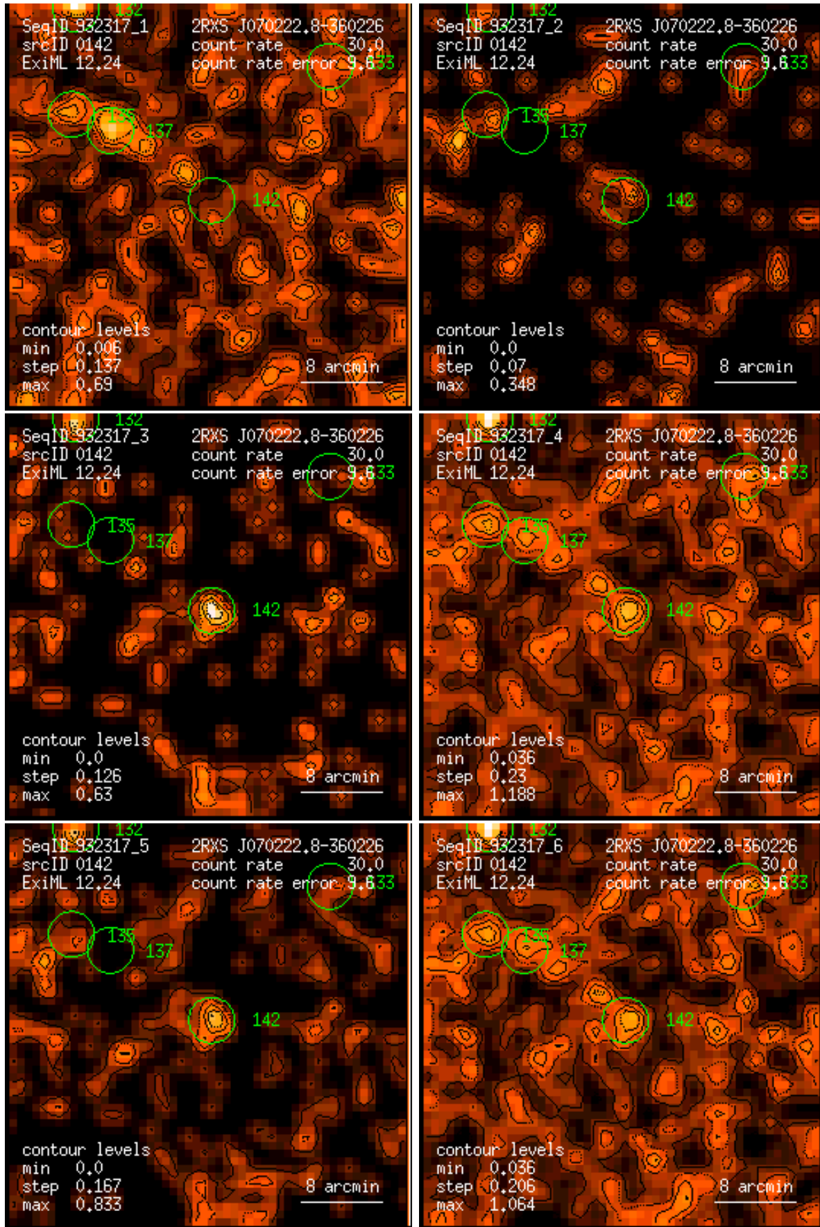
Figure 142: RASS 932317: detection 0142: band rate images, Gaussian filter: (1) PSPC channels 11 – 41, (2) 52 – 90, (3) 91 – 201, (4) 11 – 235, (5) 52 – 201, (6) 11 – 201. Broad band rates in counts/ks. Band rate contour levels in counts/ks/arcmin 2 .
