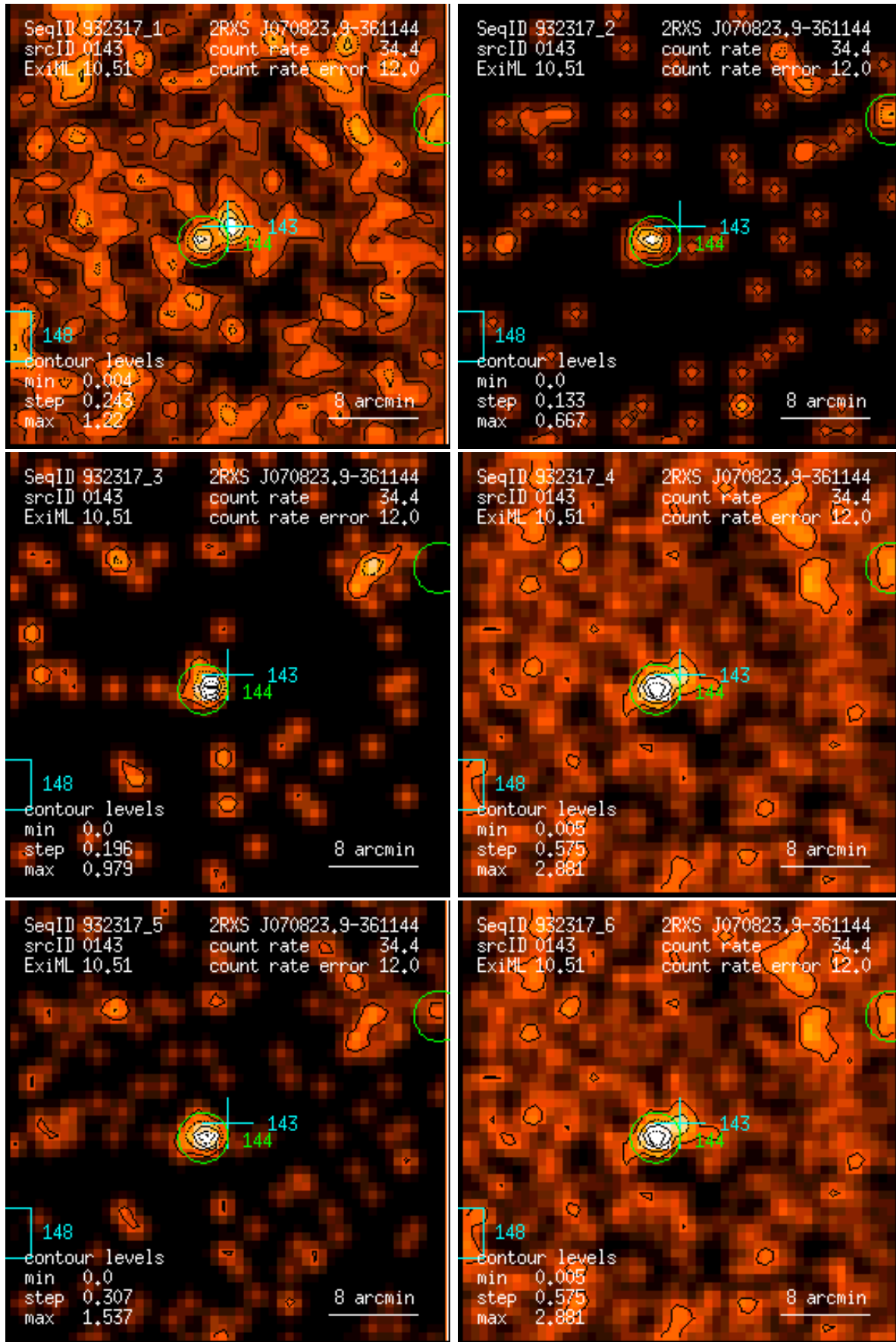
Figure 143: RASS 932317: detection 0143: band rate images, Gaussian filter: (1) PSPC channels 11 – 41, (2) 52 – 90, (3) 91 – 201, (4) 11 – 235, (5) 52 – 201, (6) 11 – 201. Broad band rates in counts/ks. Band rate contour levels in counts/ks/arcmin 2 .
