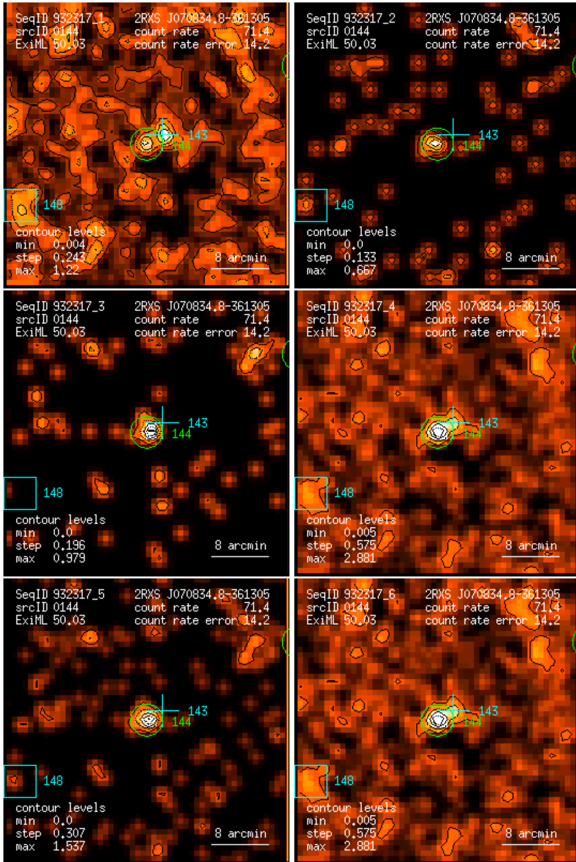
Figure 144: RASS 932317: detection 0144: band rate images, Gaussian filter: (1) PSPC channels 11 – 41, (2) 52 – 90, (3) 91 – 201, (4) 11 – 235, (5) 52 – 201, (6) 11 – 201. Broad band rates in counts/ks. Band rate contour levels in counts/ks/arcmin 2 .
