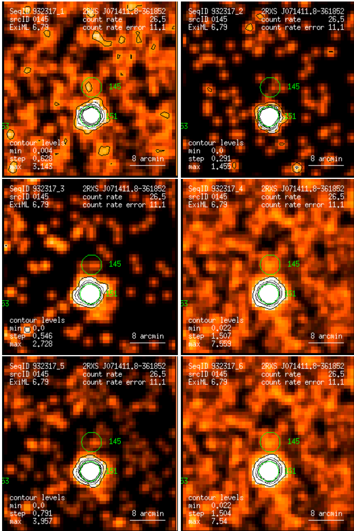
Figure 145: RASS 932317: detection 0145: band rate images, Gaussian filter: (1) PSPC channels 11 – 41, (2) 52 – 90, (3) 91 – 201, (4) 11 – 235, (5) 52 – 201, (6) 11 – 201. Broad band rates in counts/ks. Band rate contour levels in counts/ks/arcmin 2 .
