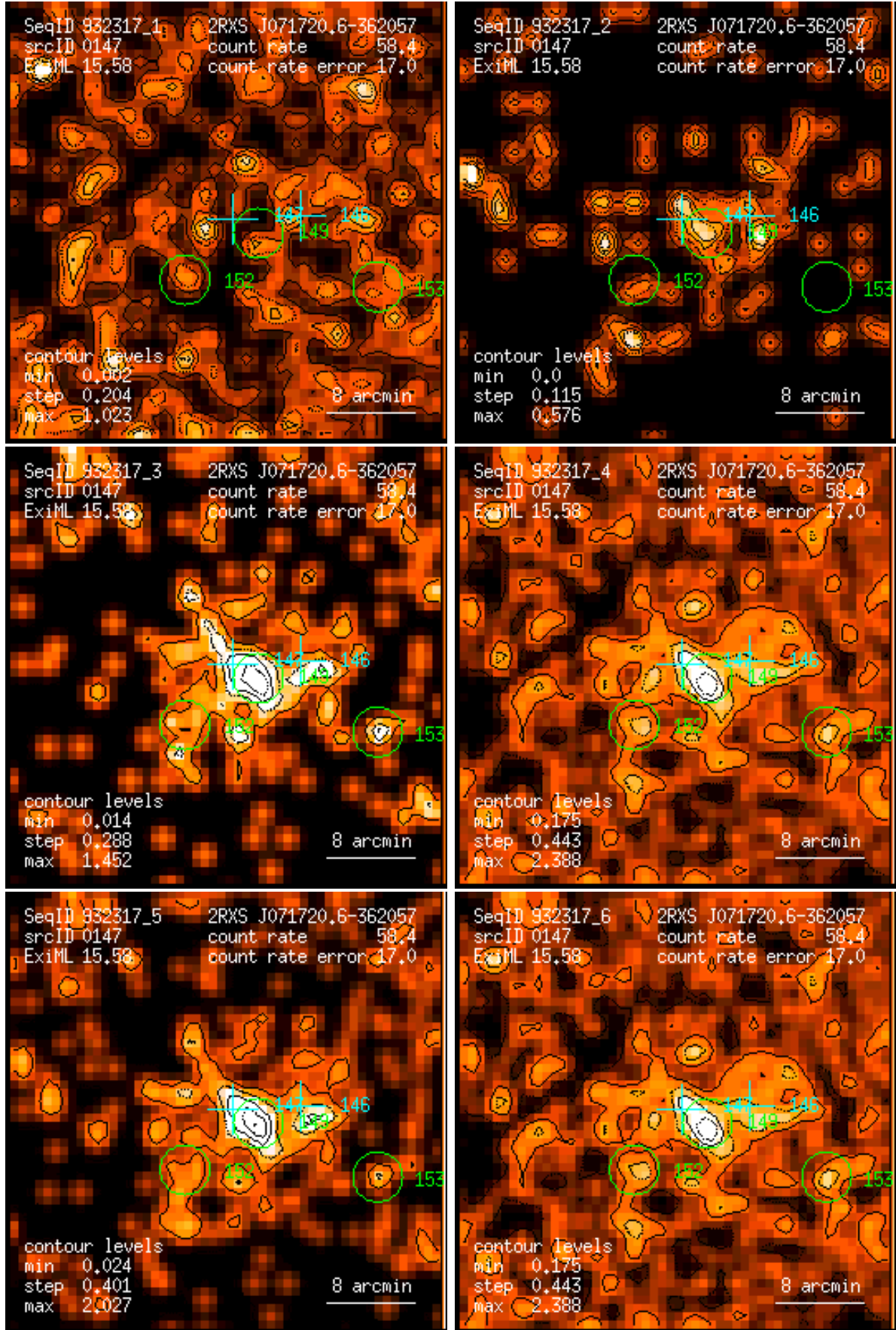
Figure 147: RASS 932317: detection 0147: band rate images, Gaussian filter: (1) PSPC channels 11 – 41, (2) 52 – 90, (3) 91 – 201, (4) 11 – 235, (5) 52 – 201, (6) 11 – 201. Broad band rates in counts/ks. Band rate contour levels in counts/ks/arcmin 2 .
