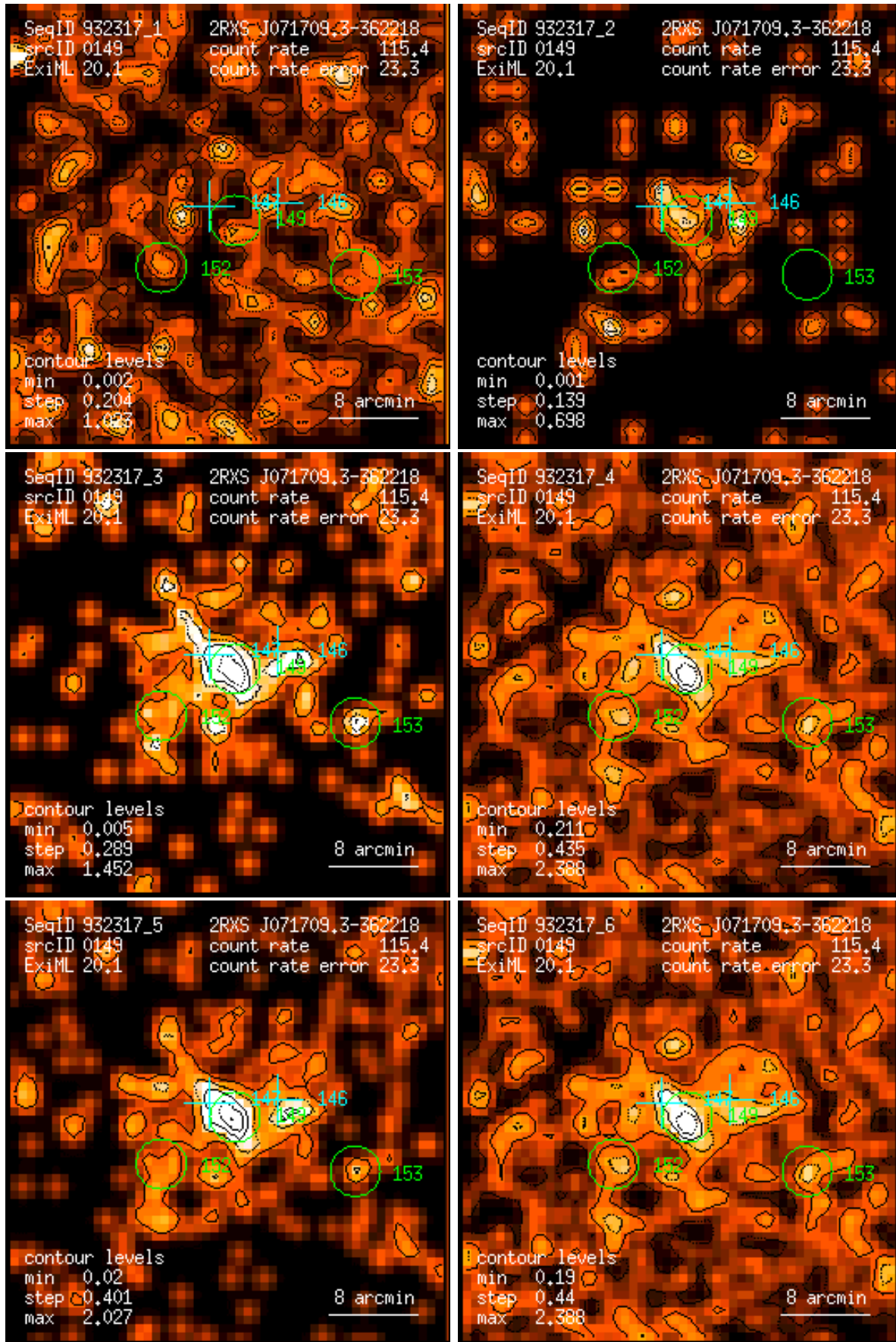
Figure 149: RASS 932317: detection 0149: band rate images, Gaussian filter: (1) PSPC channels 11 – 41, (2) 52 – 90, (3) 91 – 201, (4) 11 – 235, (5) 52 – 201, (6) 11 – 201. Broad band rates in counts/ks. Band rate contour levels in counts/ks/arcmin 2 .
