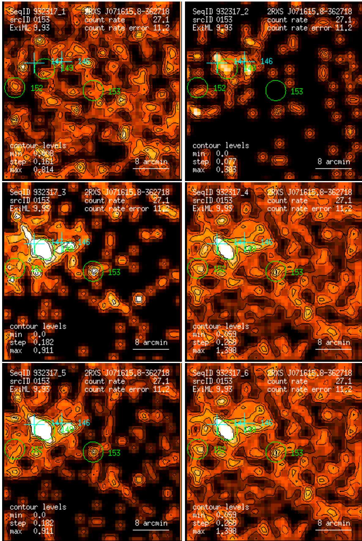
Figure 153: RASS 932317: detection 0153: band rate images, Gaussian filter: (1) PSPC channels 11 – 41, (2) 52 – 90, (3) 91 – 201, (4) 11 – 235, (5) 52 – 201, (6) 11 – 201. Broad band rates in counts/ks. Band rate contour levels in counts/ks/arcmin 2 .
