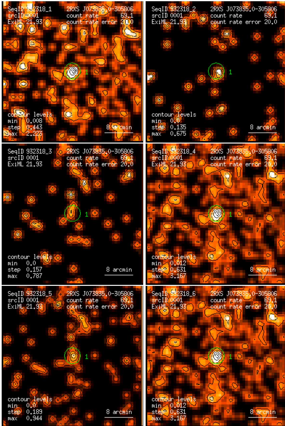
Figure 1: RASS 932318: detection 0001: band rate images, Gaussian filter: (1) PSPC channels 11 – 41, (2) 52 – 90, (3) 91 – 201, (4) 11 – 235, (5) 52 – 201, (6) 11 – 201. Broad band rates in counts/ks. Band rate contour levels in counts/ks/arcmin 2 .
