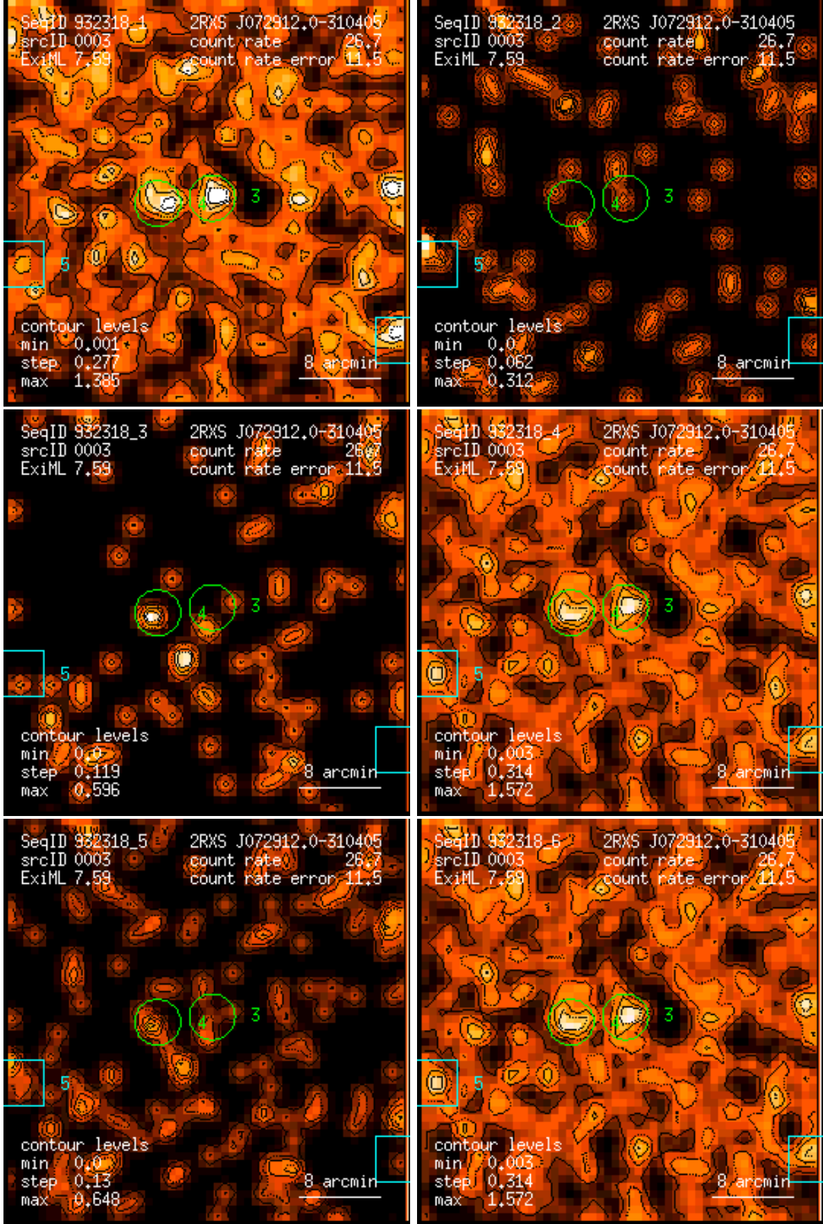
Figure 3: RASS 932318: detection 0003: band rate images, Gaussian filter: (1) PSPC channels 11 – 41, (2) 52 – 90, (3) 91 – 201, (4) 11 – 235, (5) 52 – 201, (6) 11 – 201. Broad band rates in counts/ks. Band rate contour levels in counts/ks/arcmin 2 .
