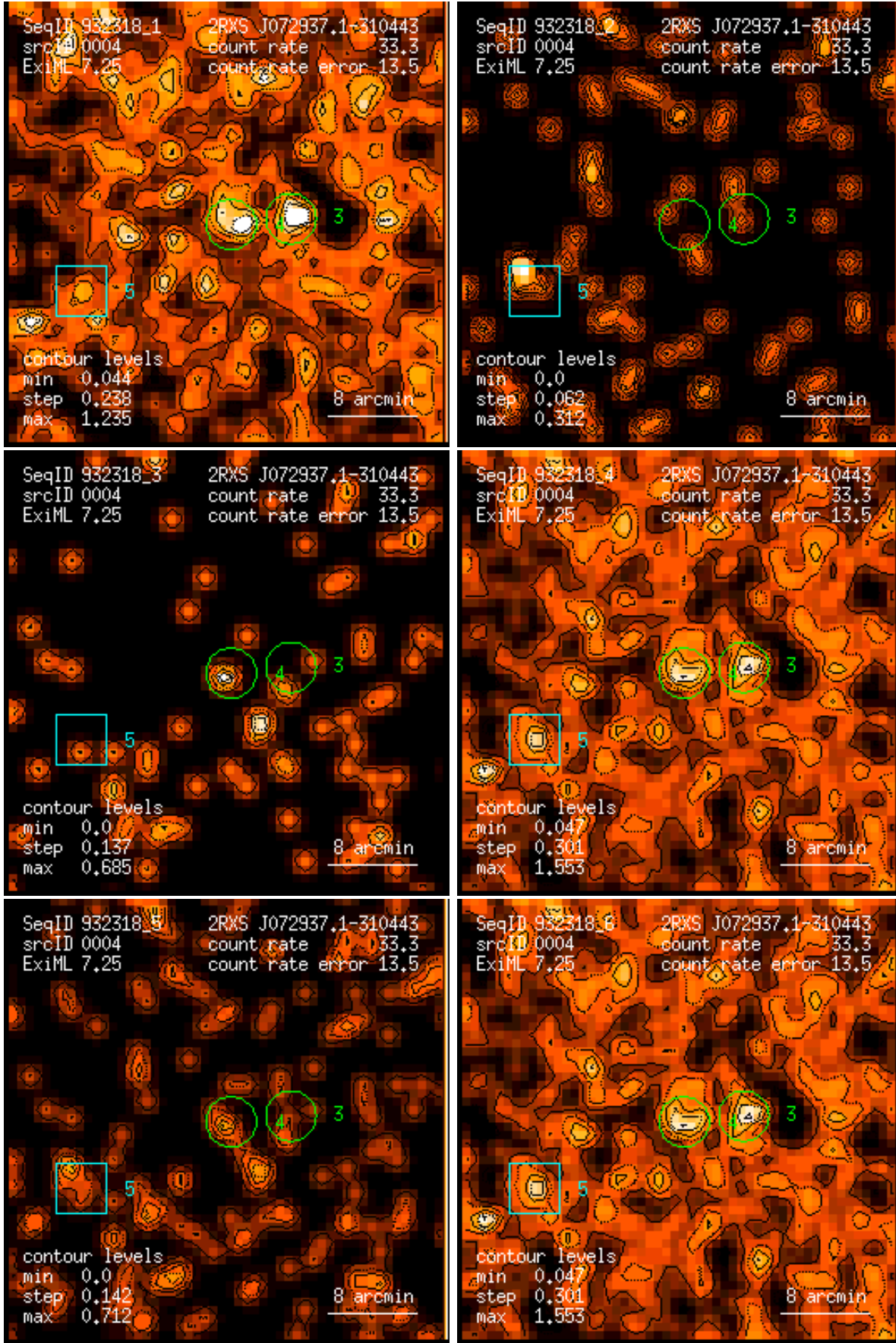
Figure 4: RASS 932318: detection 0004: band rate images, Gaussian filter: (1) PSPC channels 11 – 41, (2) 52 – 90, (3) 91 – 201, (4) 11 – 235, (5) 52 – 201, (6) 11 – 201. Broad band rates in counts/ks. Band rate contour levels in counts/ks/arcmin 2 .
