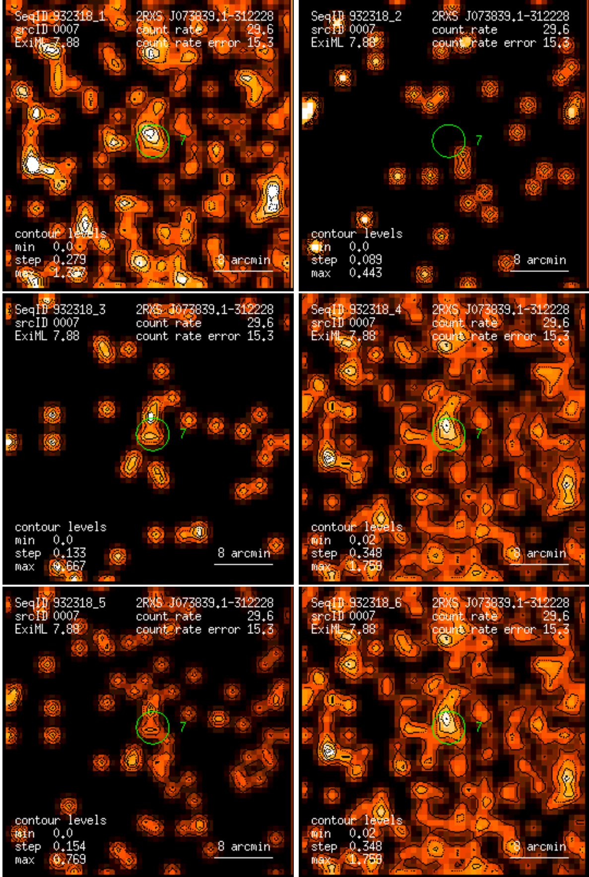
Figure 7: RASS 932318: detection 0007: band rate images, Gaussian filter: (1) PSPC channels 11 – 41, (2) 52 – 90, (3) 91 – 201, (4) 11 – 235, (5) 52 – 201, (6) 11 – 201. Broad band rates in counts/ks. Band rate contour levels in counts/ks/arcmin 2 .
