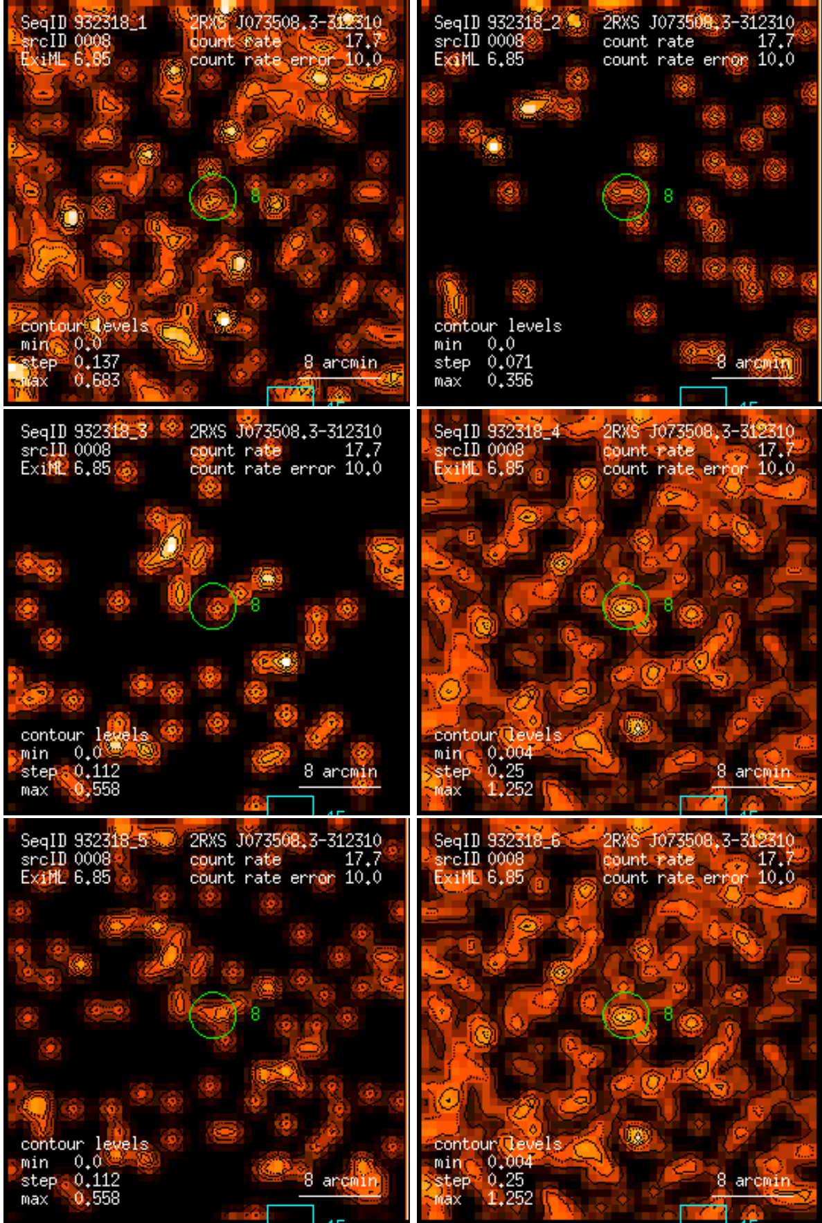
Figure 8: RASS 932318: detection 0008: band rate images, Gaussian filter: (1) PSPC channels 11 – 41, (2) 52 – 90, (3) 91 – 201, (4) 11 – 235, (5) 52 – 201, (6) 11 – 201. Broad band rates in counts/ks. Band rate contour levels in counts/ks/arcmin 2 .
