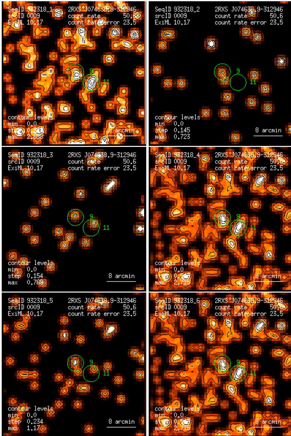
Figure 9: RASS 932318: detection 0009: band rate images, Gaussian filter: (1) PSPC channels 11 – 41, (2) 52 – 90, (3) 91 – 201, (4) 11 – 235, (5) 52 – 201, (6) 11 – 201. Broad band rates in counts/ks. Band rate contour levels in counts/ks/arcmin 2 .
