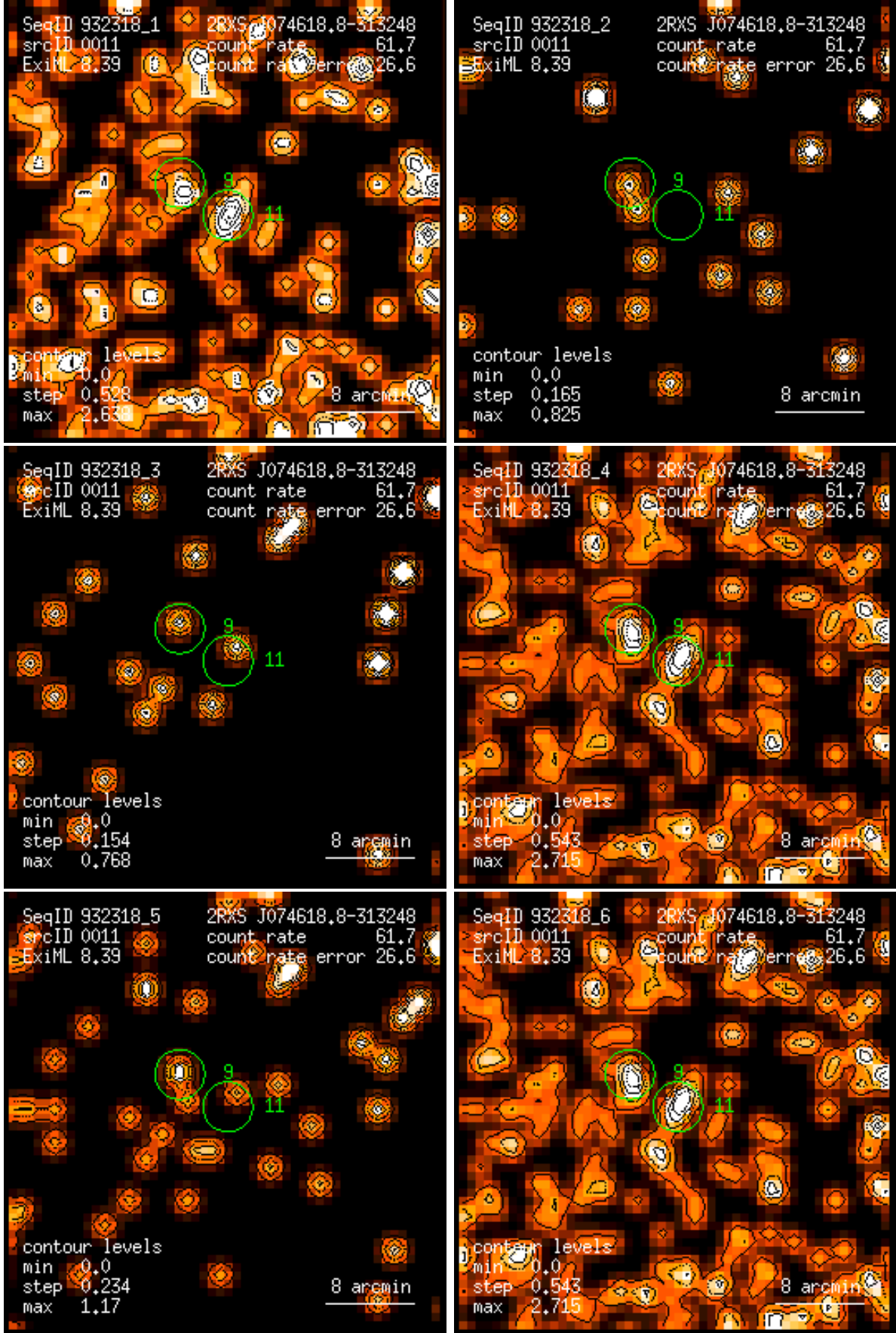
Figure 11: RASS 932318: detection 0011: band rate images, Gaussian filter: (1) PSPC channels 11 – 41, (2) 52 – 90, (3) 91 – 201, (4) 11 – 235, (5) 52 – 201, (6) 11 – 201. Broad band rates in counts/ks. Band rate contour levels in counts/ks/arcmin 2 .
