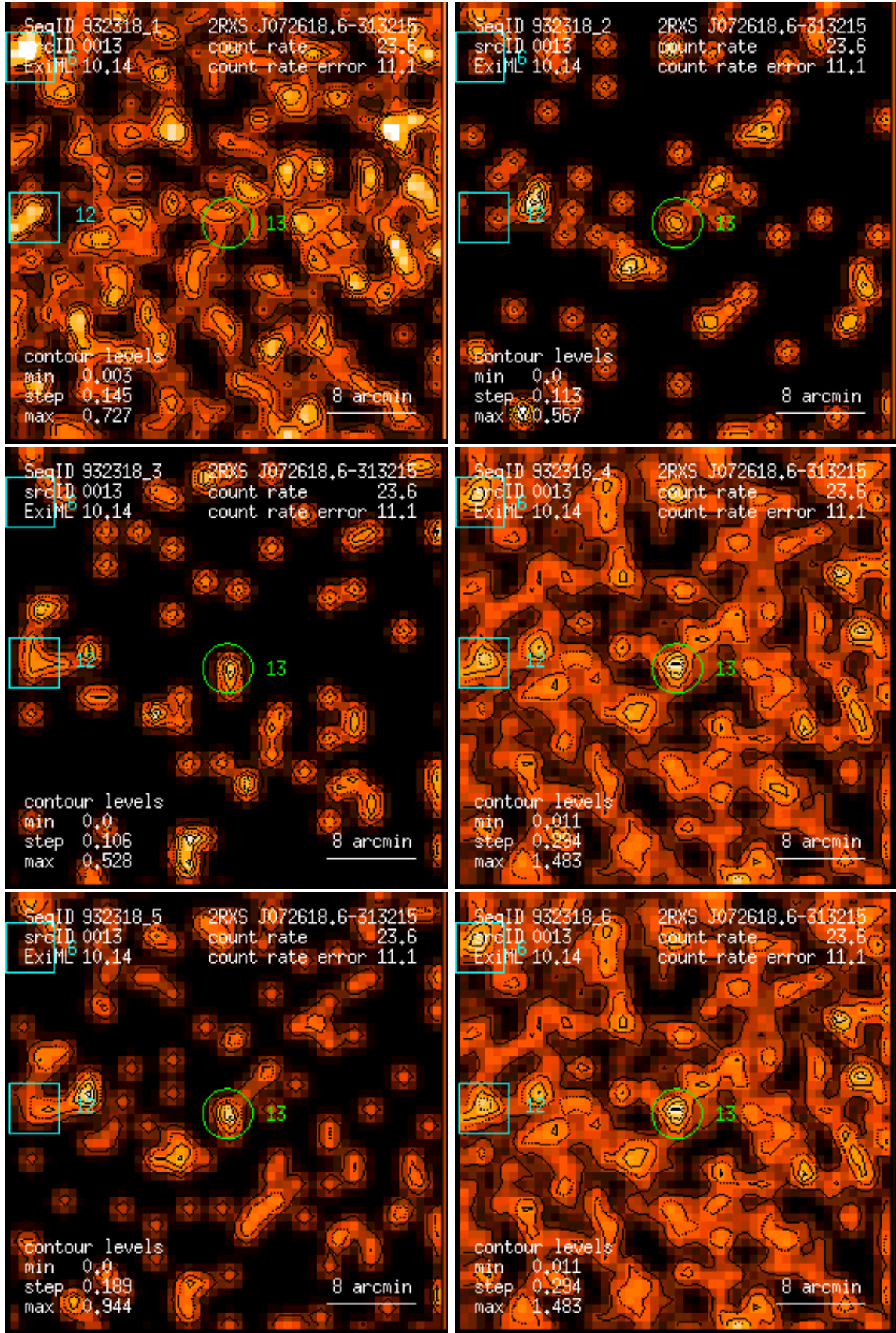
Figure 13: RASS 932318: detection 0013: band rate images, Gaussian filter: (1) PSPC channels 11 – 41, (2) 52 – 90, (3) 91 – 201, (4) 11 – 235, (5) 52 – 201, (6) 11 – 201. Broad band rates in counts/ks. Band rate contour levels in counts/ks/arcmin 2 .
