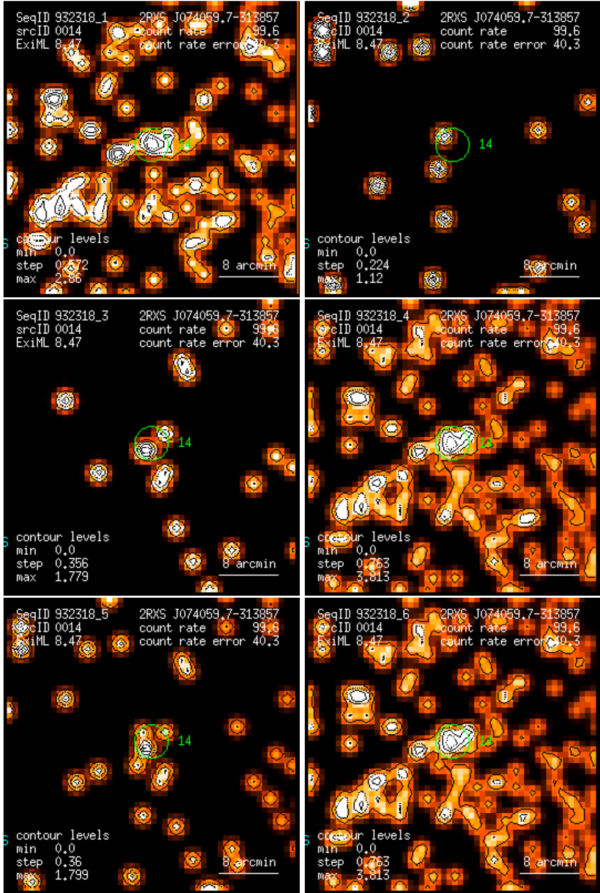
Figure 14: RASS 932318: detection 0014: band rate images, Gaussian filter: (1) PSPC channels 11 – 41, (2) 52 – 90, (3) 91 – 201, (4) 11 – 235, (5) 52 – 201, (6) 11 – 201. Broad band rates in counts/ks. Band rate contour levels in counts/ks/arcmin 2 .
