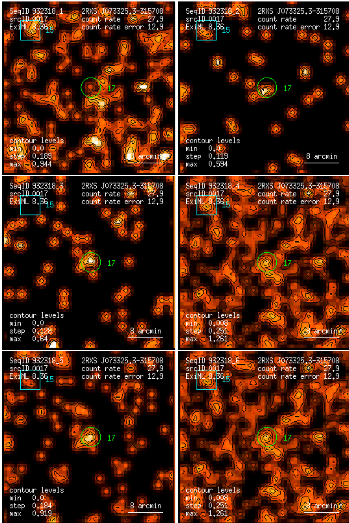
Figure 17: RASS 932318: detection 0017: band rate images, Gaussian filter: (1) PSPC channels 11 – 41, (2) 52 – 90, (3) 91 – 201, (4) 11 – 235, (5) 52 – 201, (6) 11 – 201. Broad band rates in counts/ks. Band rate contour levels in counts/ks/arcmin 2 .
