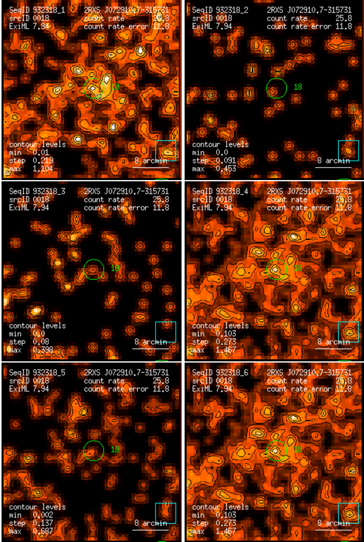
Figure 18: RASS 932318: detection 0018: band rate images, Gaussian filter: (1) PSPC channels 11 – 41, (2) 52 – 90, (3) 91 – 201, (4) 11 – 235, (5) 52 – 201, (6) 11 – 201. Broad band rates in counts/ks. Band rate contour levels in counts/ks/arcmin 2 .
