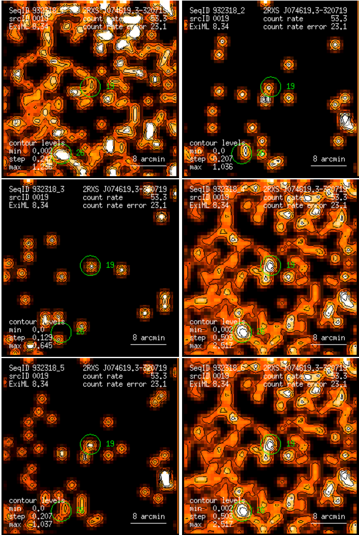
Figure 19: RASS 932318: detection 0019: band rate images, Gaussian filter: (1) PSPC channels 11 – 41, (2) 52 – 90, (3) 91 – 201, (4) 11 – 235, (5) 52 – 201, (6) 11 – 201. Broad band rates in counts/ks. Band rate contour levels in counts/ks/arcmin 2 .
