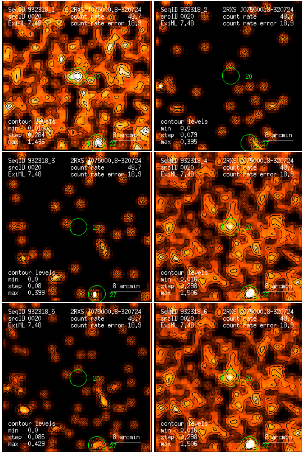
Figure 20: RASS 932318: detection 0020: band rate images, Gaussian filter: (1) PSPC channels 11 – 41, (2) 52 – 90, (3) 91 – 201, (4) 11 – 235, (5) 52 – 201, (6) 11 – 201. Broad band rates in counts/ks. Band rate contour levels in counts/ks/arcmin 2 .
