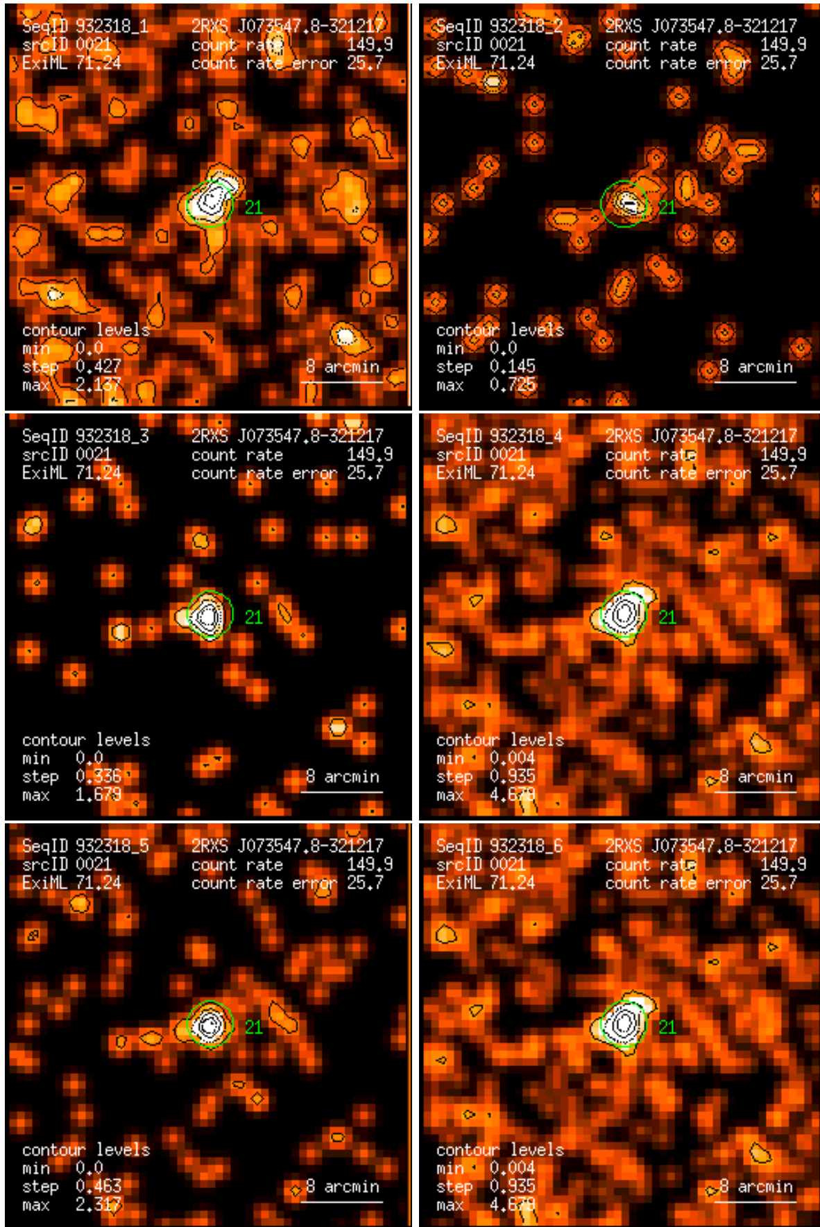
Figure 21: RASS 932318: detection 0021: band rate images, Gaussian filter: (1) PSPC channels 11 – 41, (2) 52 – 90, (3) 91 – 201, (4) 11 – 235, (5) 52 – 201, (6) 11 – 201. Broad band rates in counts/ks. Band rate contour levels in counts/ks/arcmin 2 .
