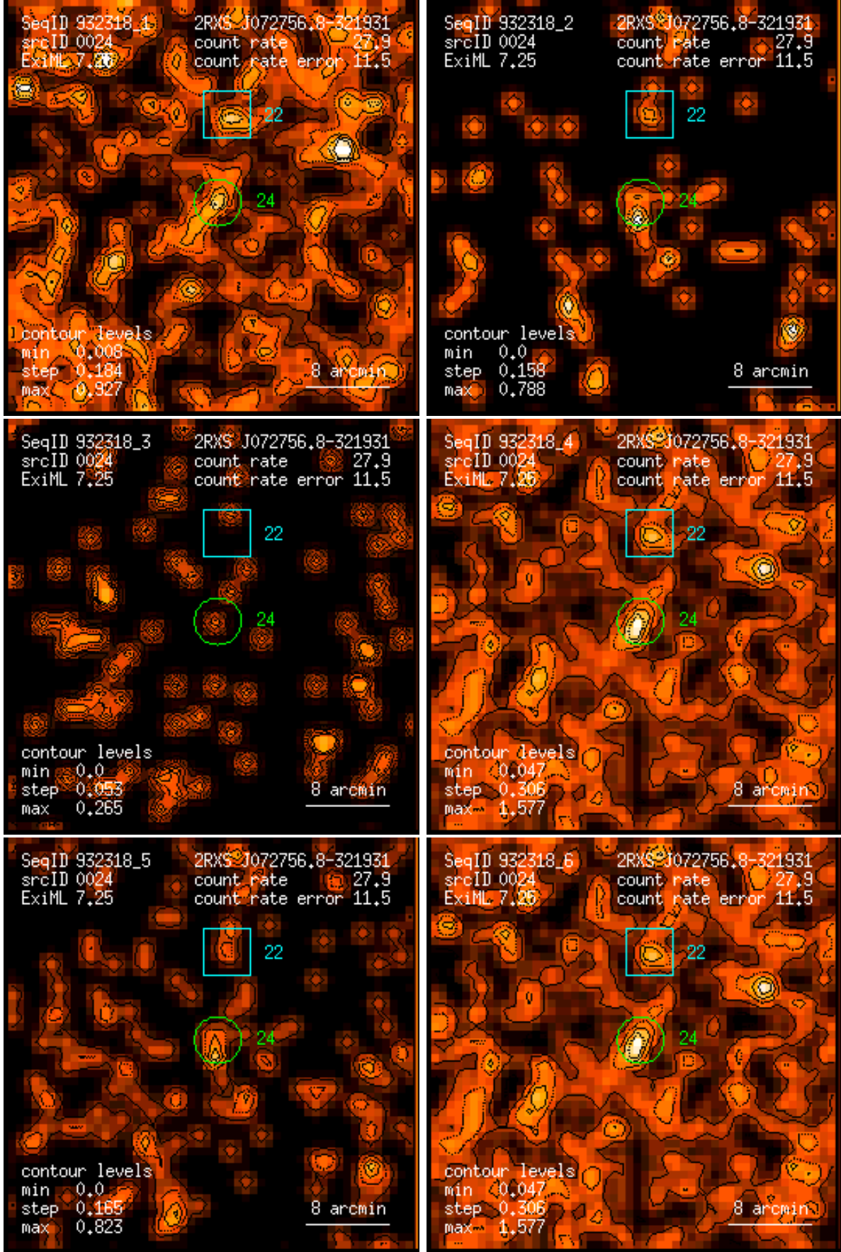
Figure 24: RASS 932318: detection 0024: band rate images, Gaussian filter: (1) PSPC channels 11 – 41, (2) 52 – 90, (3) 91 – 201, (4) 11 – 235, (5) 52 – 201, (6) 11 – 201. Broad band rates in counts/ks. Band rate contour levels in counts/ks/arcmin 2 .
