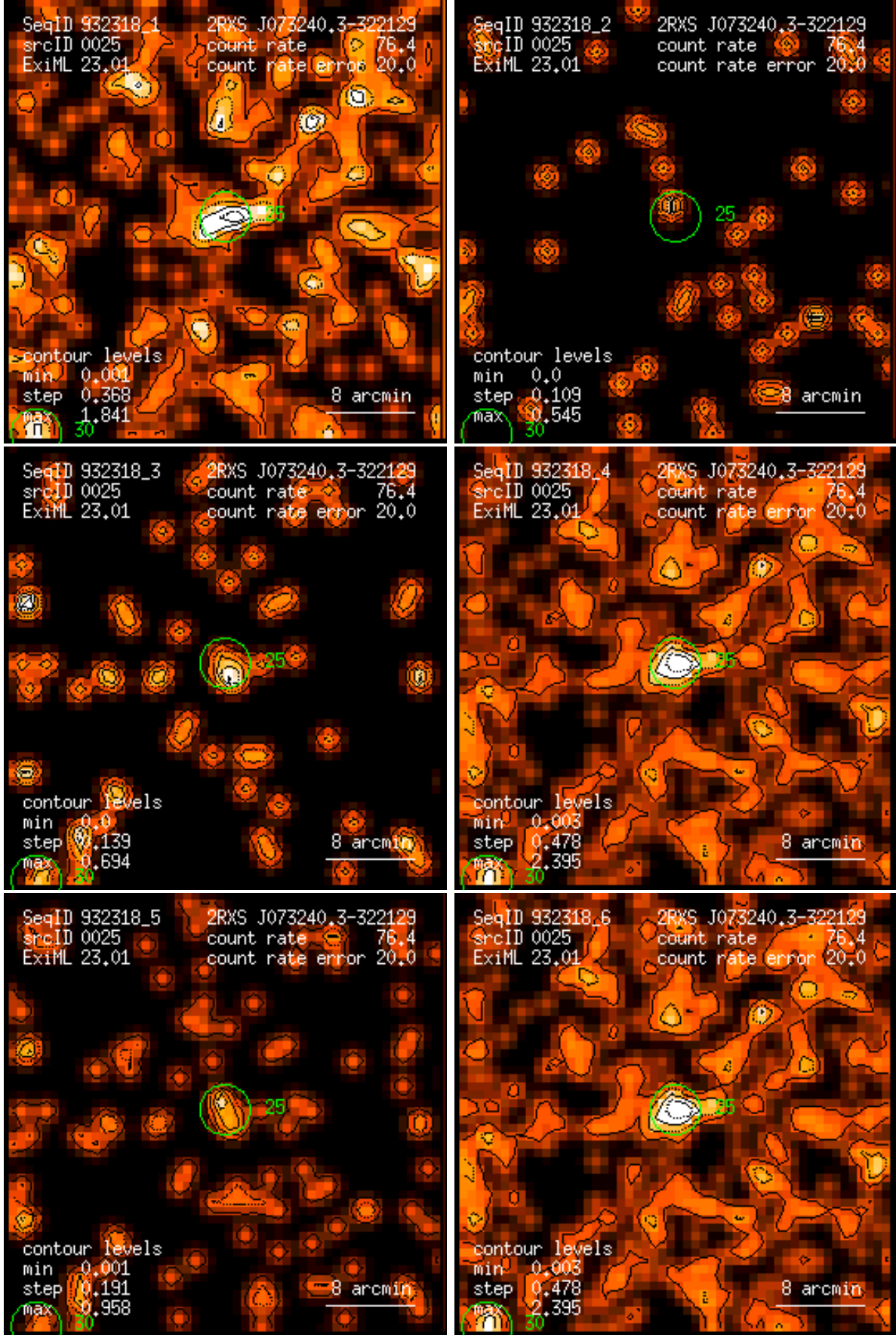
Figure 25: RASS 932318: detection 0025: band rate images, Gaussian filter: (1) PSPC channels 11 – 41, (2) 52 – 90, (3) 91 – 201, (4) 11 – 235, (5) 52 – 201, (6) 11 – 201. Broad band rates in counts/ks. Band rate contour levels in counts/ks/arcmin 2 .
